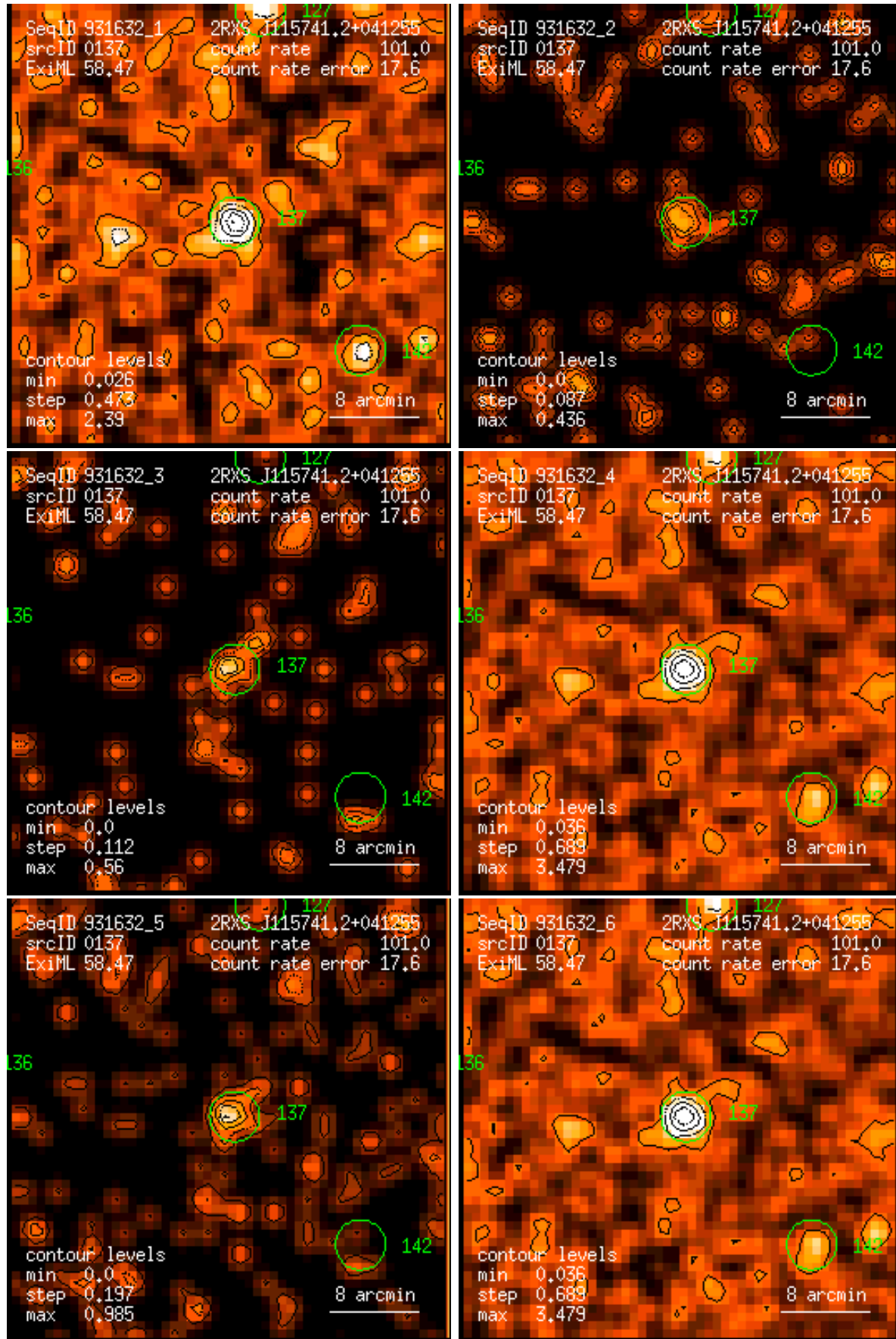
Figure 137: RASS 931632: detection 0137: band rate images, Gaussian filter: (1) PSPC channels 11 – 41, (2) 52 – 90, (3) 91 – 201, (4) 11 – 235, (5) 52 – 201, (6) 11 – 201. Broad band rates in counts/ks. Band rate contour levels in counts/ks/arcmin 2 .
