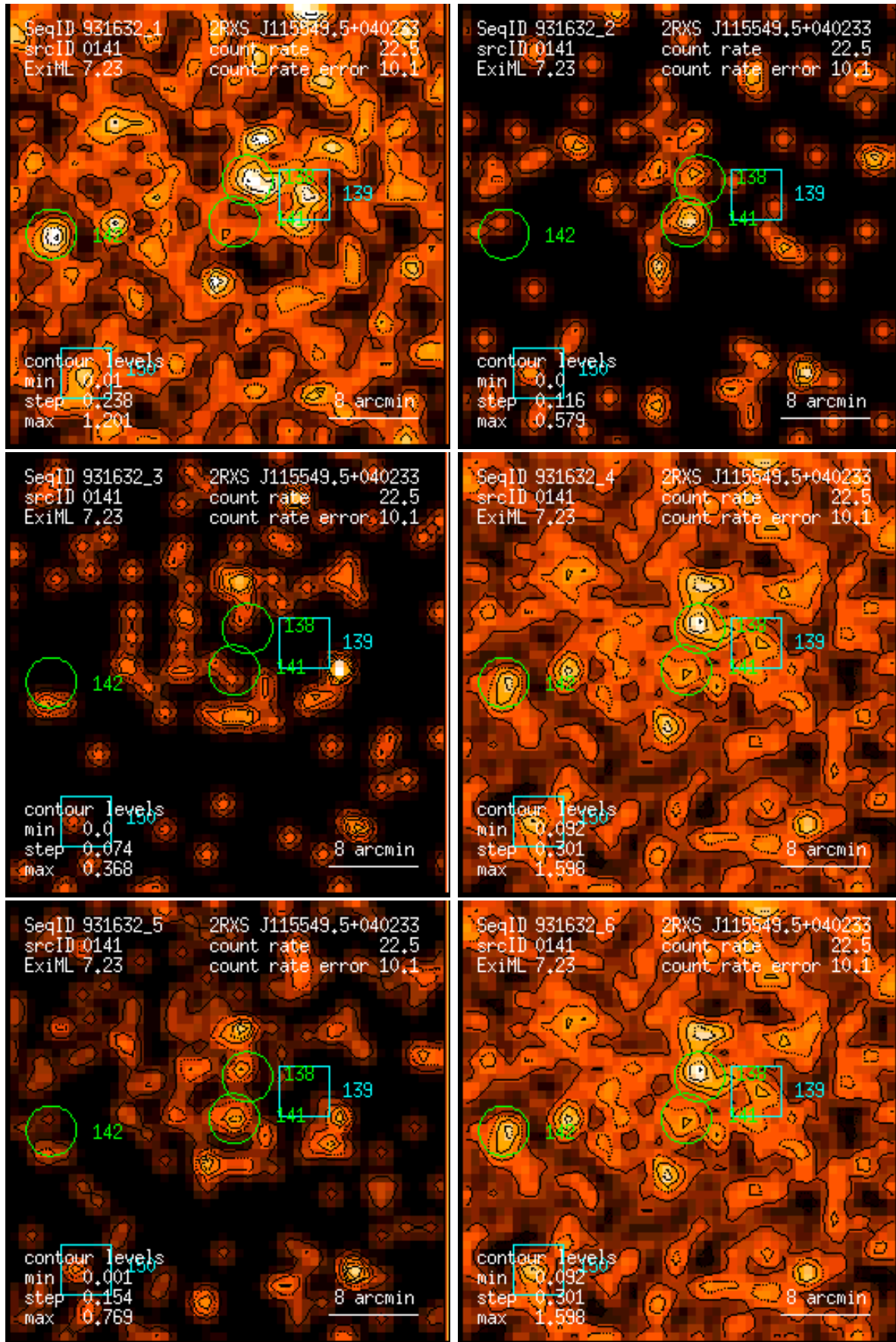
Figure 141: RASS 931632: detection 0141: band rate images, Gaussian filter: (1) PSPC channels 11 – 41, (2) 52 – 90, (3) 91 – 201, (4) 11 – 235, (5) 52 – 201, (6) 11 – 201. Broad band rates in counts/ks. Band rate contour levels in counts/ks/arcmin 2 .
