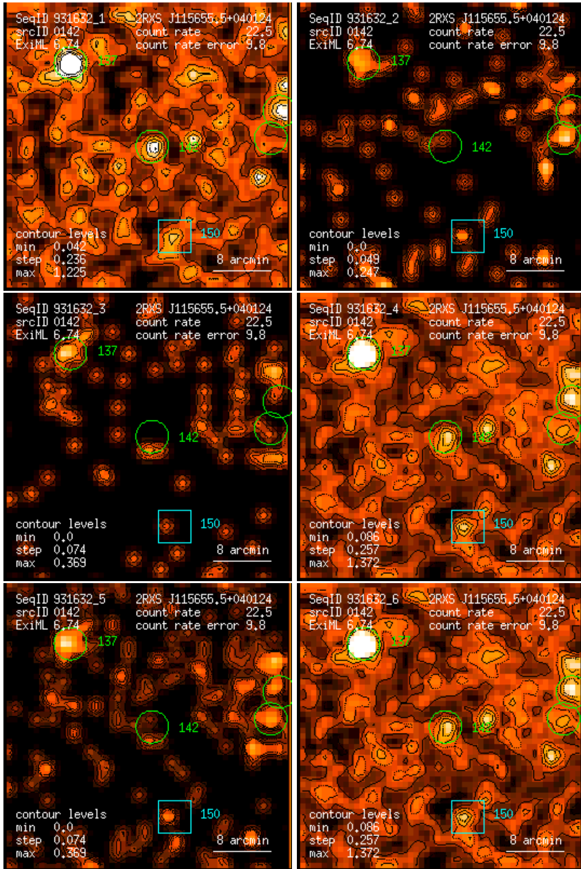
Figure 142: RASS 931632: detection 0142: band rate images, Gaussian filter: (1) PSPC channels 11 – 41, (2) 52 – 90, (3) 91 – 201, (4) 11 – 235, (5) 52 – 201, (6) 11 – 201. Broad band rates in counts/ks. Band rate contour levels in counts/ks/arcmin 2 .
