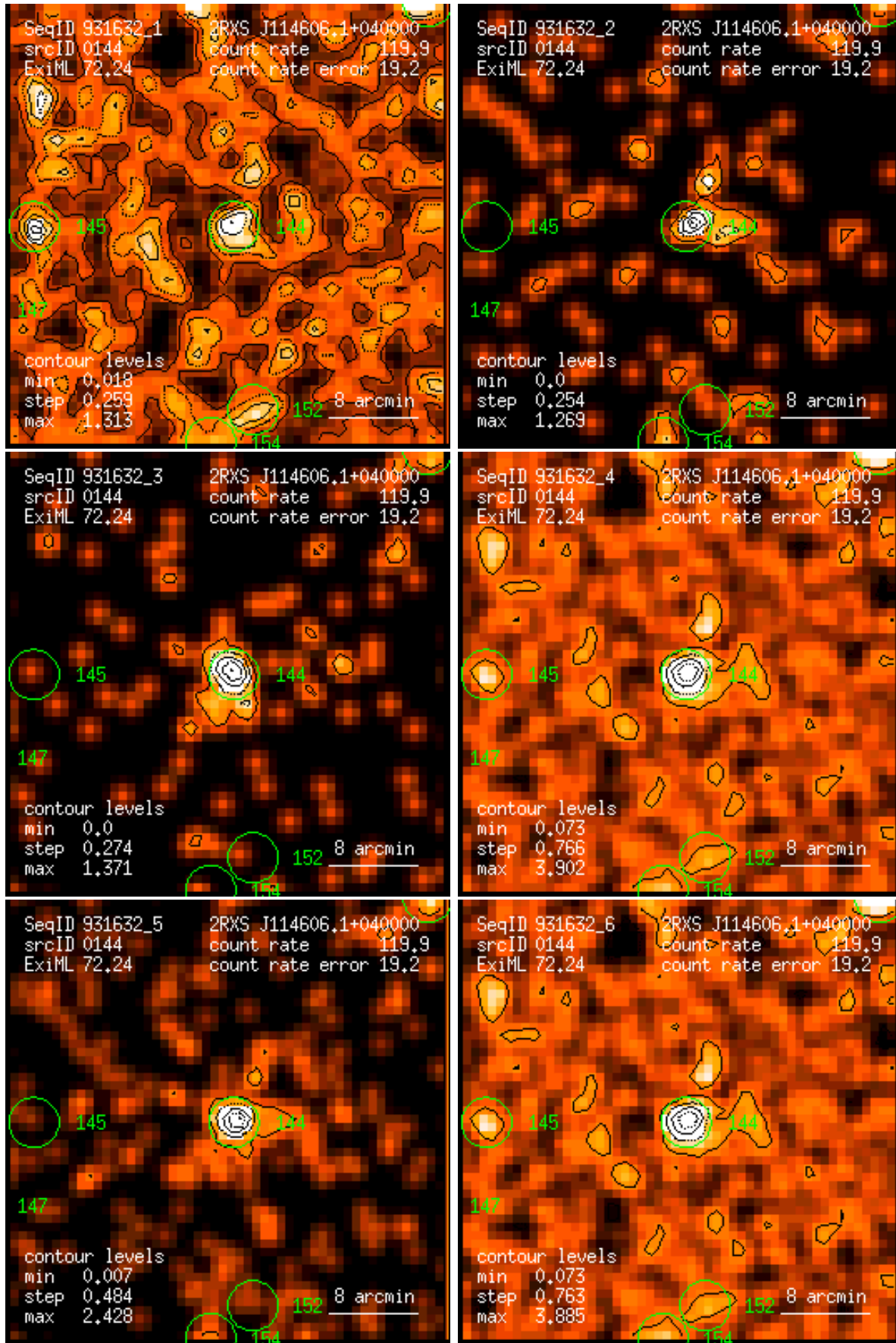
Figure 144: RASS 931632: detection 0144: band rate images, Gaussian filter: (1) PSPC channels 11 – 41, (2) 52 – 90, (3) 91 – 201, (4) 11 – 235, (5) 52 – 201, (6) 11 – 201. Broad band rates in counts/ks. Band rate contour levels in counts/ks/arcmin 2 .
