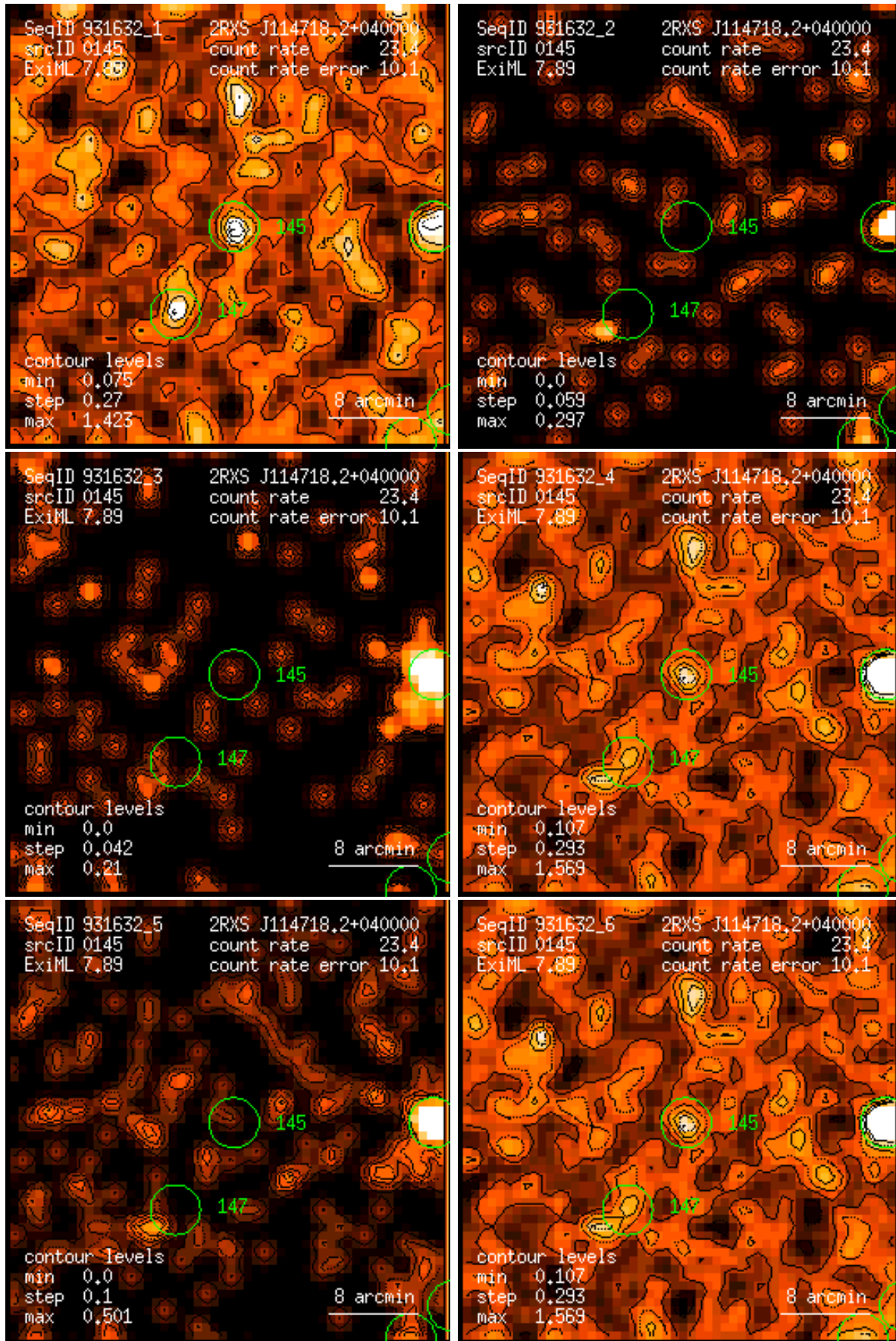
Figure 145: RASS 931632: detection 0145: band rate images, Gaussian filter: (1) PSPC channels 11 – 41, (2) 52 – 90, (3) 91 – 201, (4) 11 – 235, (5) 52 – 201, (6) 11 – 201. Broad band rates in counts/ks. Band rate contour levels in counts/ks/arcmin 2 .
