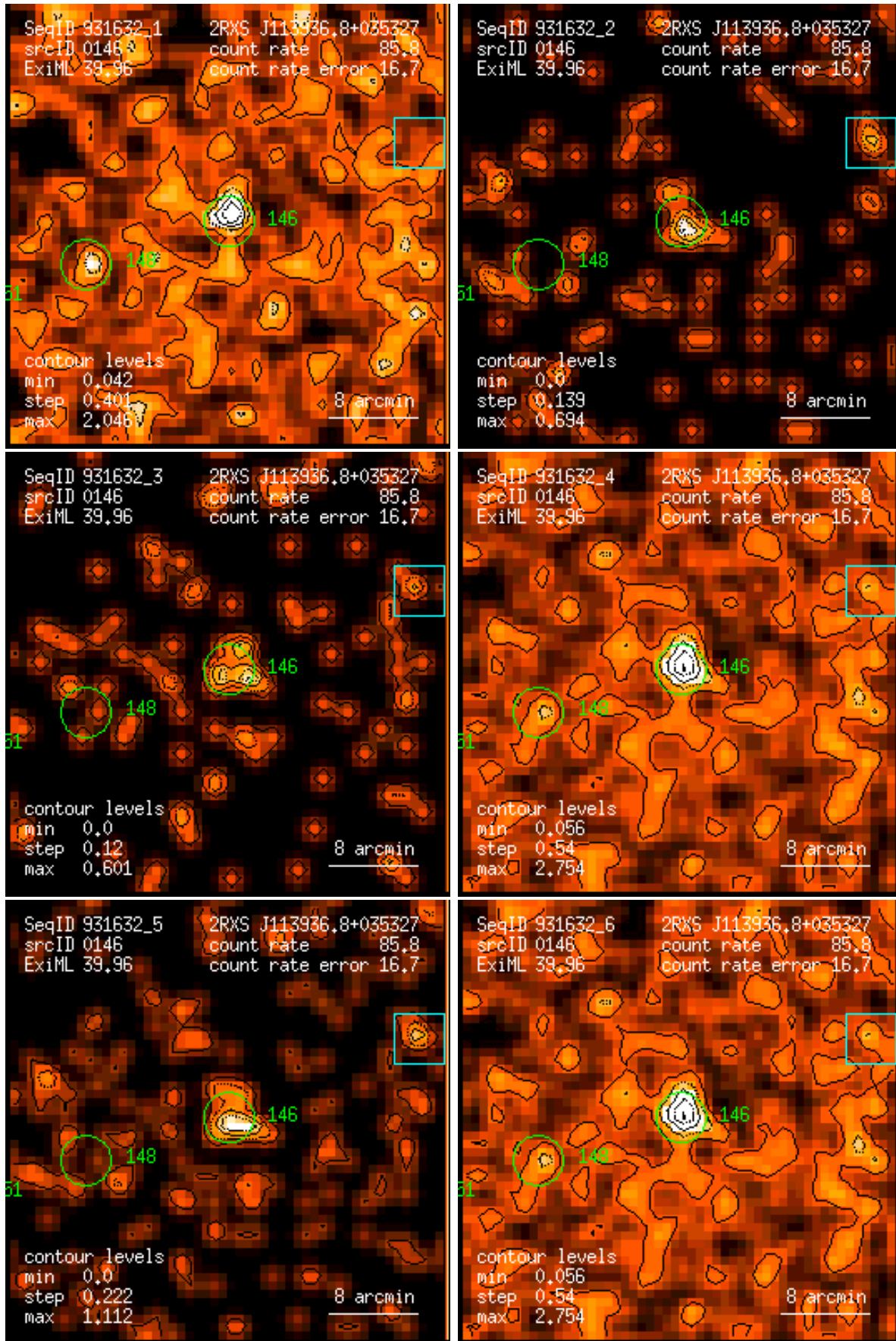
Figure 146: RASS 931632: detection 0146: band rate images, Gaussian filter: (1) PSPC channels 11 – 41, (2) 52 – 90, (3) 91 – 201, (4) 11 – 235, (5) 52 – 201, (6) 11 – 201. Broad band rates in counts/ks. Band rate contour levels in counts/ks/arcmin 2 .
