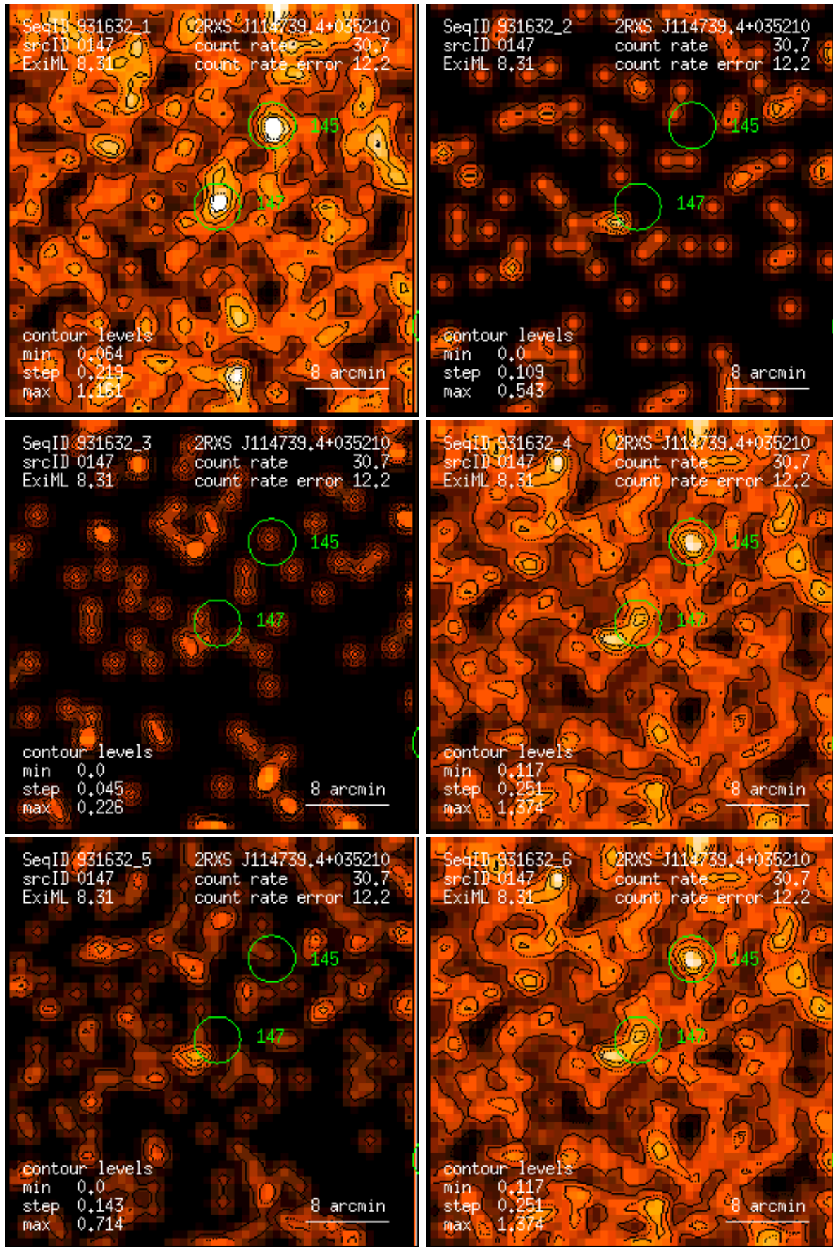
Figure 147: RASS 931632: detection 0147: band rate images, Gaussian filter: (1) PSPC channels 11 – 41, (2) 52 – 90, (3) 91 – 201, (4) 11 – 235, (5) 52 – 201, (6) 11 – 201. Broad band rates in counts/ks. Band rate contour levels in counts/ks/arcmin 2 .
