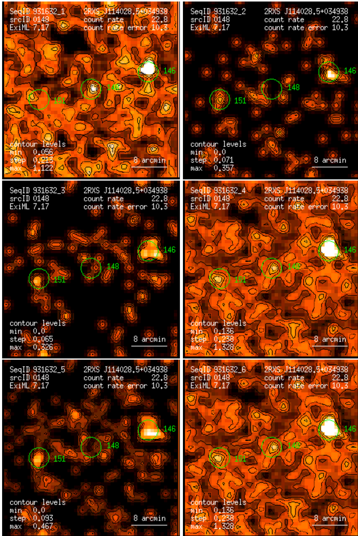
Figure 148: RASS 931632: detection 0148: band rate images, Gaussian filter: (1) PSPC channels 11 – 41, (2) 52 – 90, (3) 91 – 201, (4) 11 – 235, (5) 52 – 201, (6) 11 – 201. Broad band rates in counts/ks. Band rate contour levels in counts/ks/arcmin 2 .
