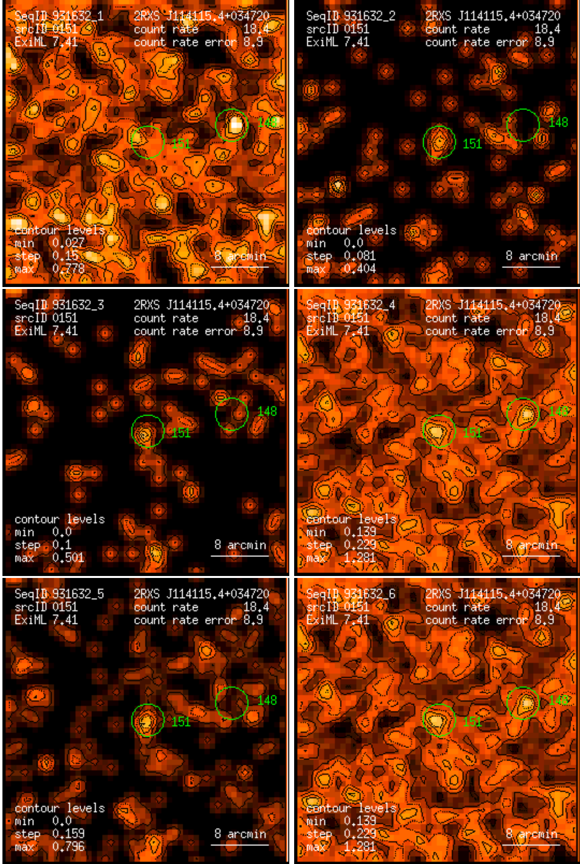
Figure 151: RASS 931632: detection 0151: band rate images, Gaussian filter: (1) PSPC channels 11 – 41, (2) 52 – 90, (3) 91 – 201, (4) 11 – 235, (5) 52 – 201, (6) 11 – 201. Broad band rates in counts/ks. Band rate contour levels in counts/ks/arcmin 2 .
