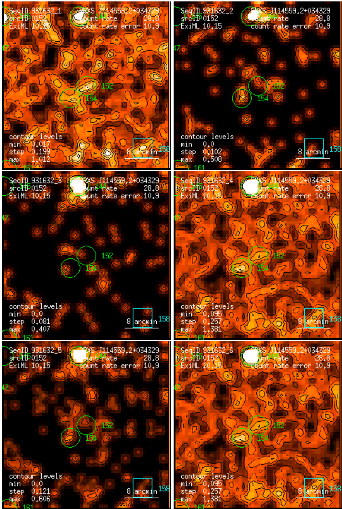
Figure 152: RASS 931632: detection 0152: band rate images, Gaussian filter: (1) PSPC channels 11 – 41, (2) 52 – 90, (3) 91 – 201, (4) 11 – 235, (5) 52 – 201, (6) 11 – 201. Broad band rates in counts/ks. Band rate contour levels in counts/ks/arcmin 2 .
