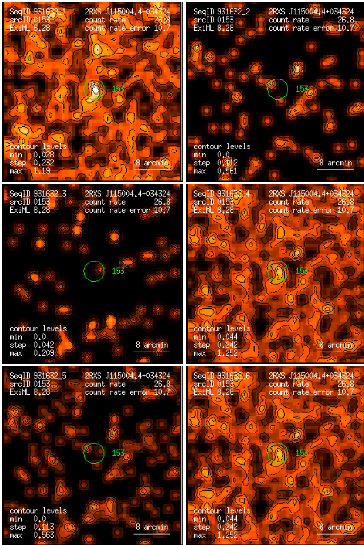
Figure 153: RASS 931632: detection 0153: band rate images, Gaussian filter: (1) PSPC channels 11 – 41, (2) 52 – 90, (3) 91 – 201, (4) 11 – 235, (5) 52 – 201, (6) 11 – 201. Broad band rates in counts/ks. Band rate contour levels in counts/ks/arcmin 2 .
