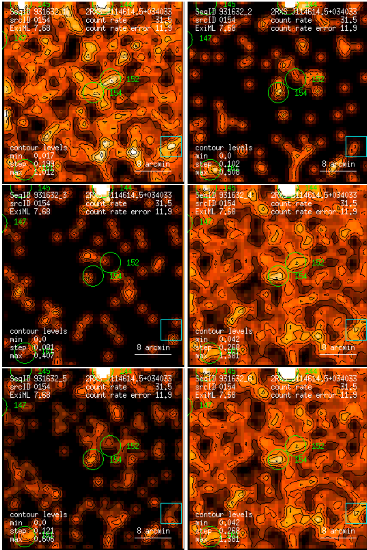
Figure 154: RASS 931632: detection 0154: band rate images, Gaussian filter: (1) PSPC channels 11 – 41, (2) 52 – 90, (3) 91 – 201, (4) 11 – 235, (5) 52 – 201, (6) 11 – 201. Broad band rates in counts/ks. Band rate contour levels in counts/ks/arcmin 2 .
