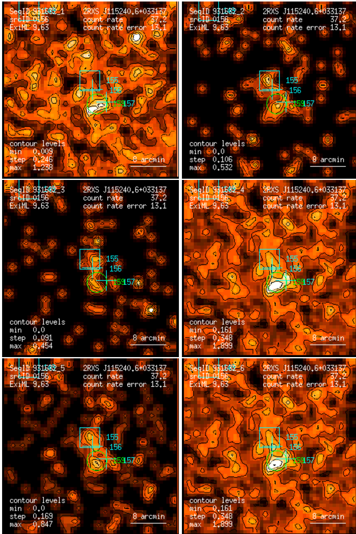
Figure 156: RASS 931632: detection 0156: band rate images, Gaussian filter: (1) PSPC channels 11 – 41, (2) 52 – 90, (3) 91 – 201, (4) 11 – 235, (5) 52 – 201, (6) 11 – 201. Broad band rates in counts/ks. Band rate contour levels in counts/ks/arcmin 2 .
