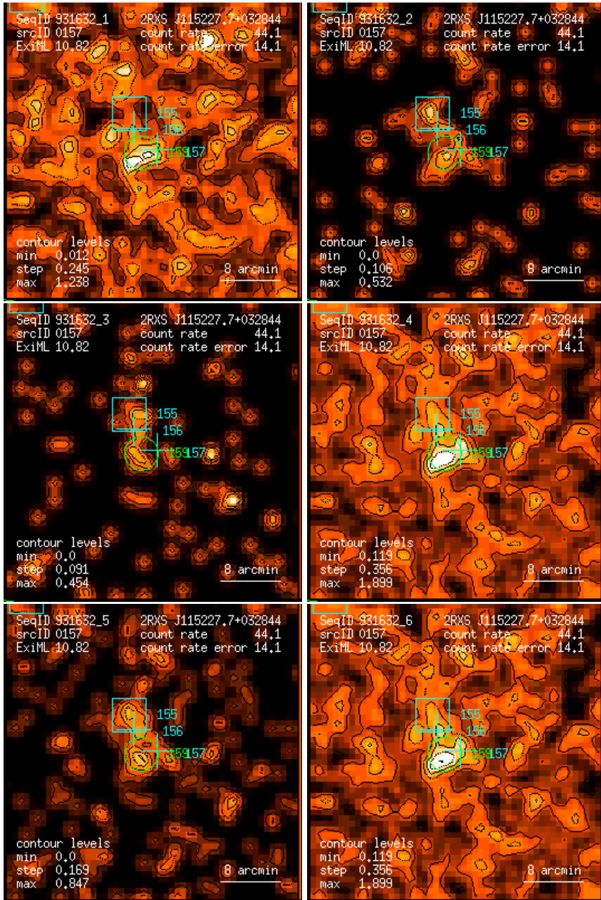
Figure 157: RASS 931632: detection 0157: band rate images, Gaussian filter: (1) PSPC channels 11 – 41, (2) 52 – 90, (3) 91 – 201, (4) 11 – 235, (5) 52 – 201, (6) 11 – 201. Broad band rates in counts/ks. Band rate contour levels in counts/ks/arcmin 2 .
