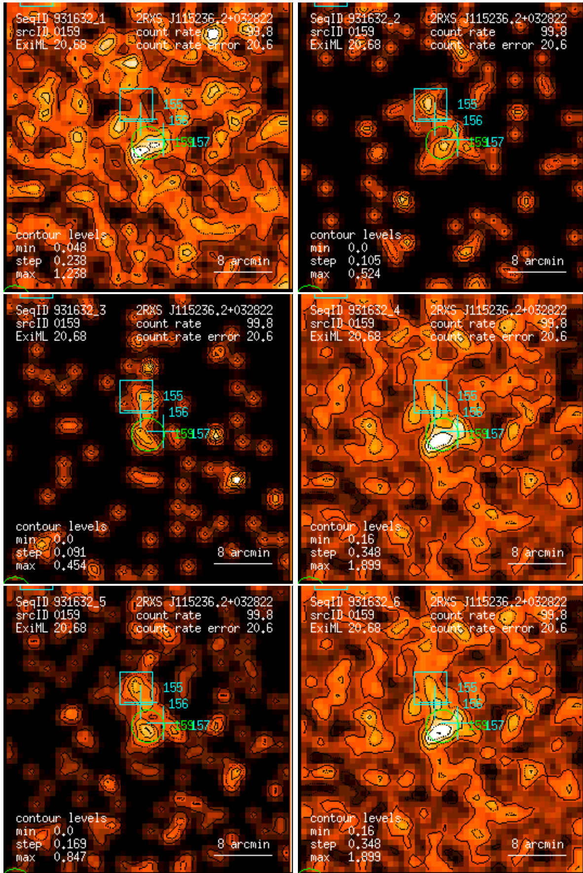
Figure 159: RASS 931632: detection 0159: band rate images, Gaussian filter: (1) PSPC channels 11 – 41, (2) 52 – 90, (3) 91 – 201, (4) 11 – 235, (5) 52 – 201, (6) 11 – 201. Broad band rates in counts/ks. Band rate contour levels in counts/ks/arcmin 2 .
