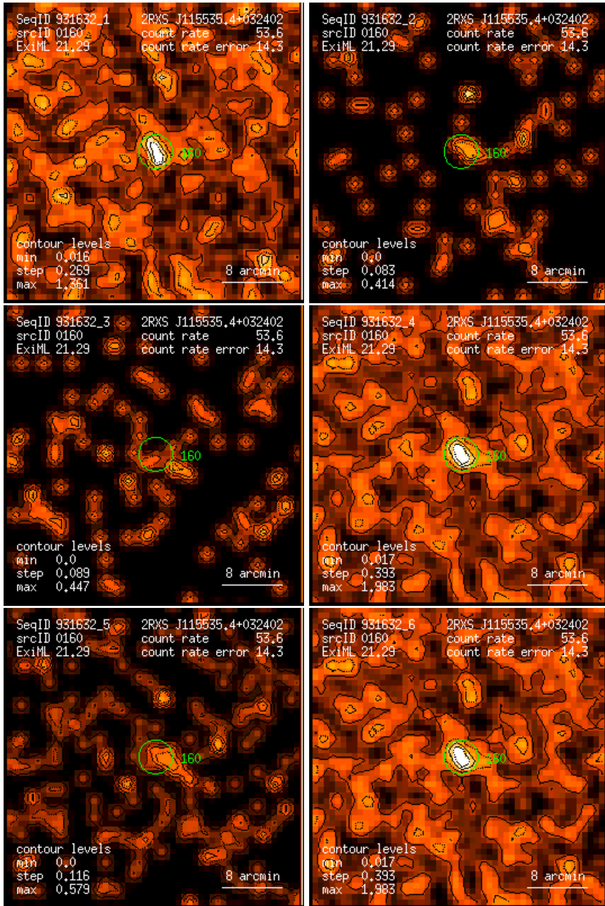
Figure 160: RASS 931632: detection 0160: band rate images, Gaussian filter: (1) PSPC channels 11 – 41, (2) 52 – 90, (3) 91 – 201, (4) 11 – 235, (5) 52 – 201, (6) 11 – 201. Broad band rates in counts/ks. Band rate contour levels in counts/ks/arcmin 2 .
