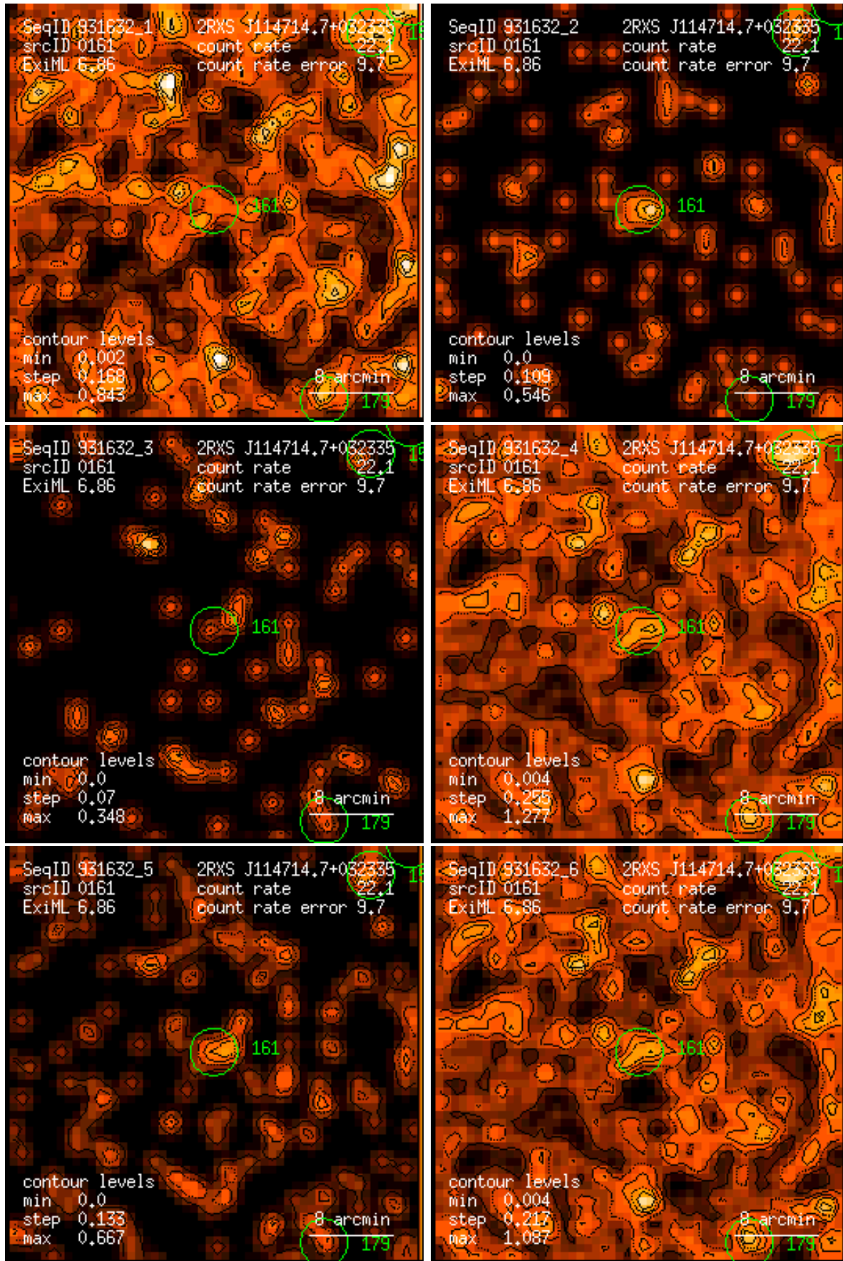
Figure 161: RASS 931632: detection 0161: band rate images, Gaussian filter: (1) PSPC channels 11 – 41, (2) 52 – 90, (3) 91 – 201, (4) 11 – 235, (5) 52 – 201, (6) 11 – 201. Broad band rates in counts/ks. Band rate contour levels in counts/ks/arcmin 2 .
