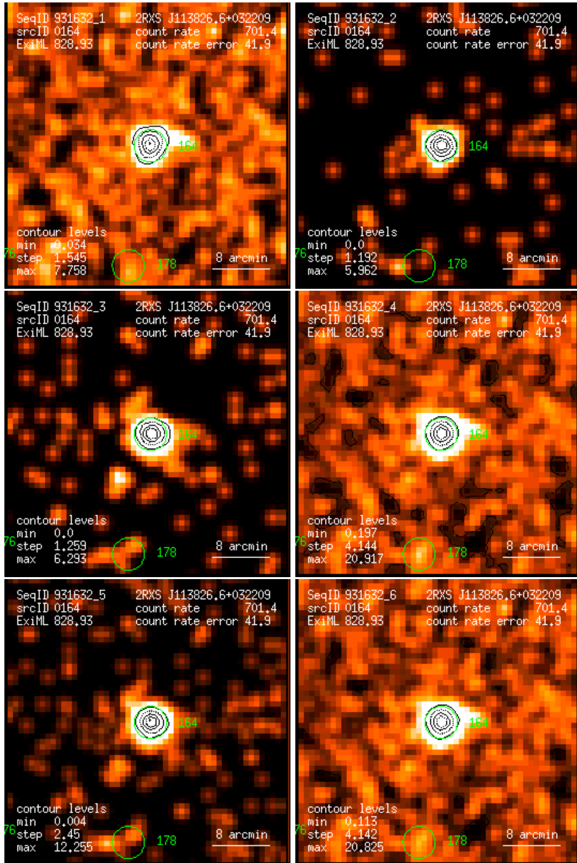
Figure 164: RASS 931632: detection 0164: band rate images, Gaussian filter: (1) PSPC channels 11 – 41, (2) 52 – 90, (3) 91 – 201, (4) 11 – 235, (5) 52 – 201, (6) 11 – 201. Broad band rates in counts/ks. Band rate contour levels in counts/ks/arcmin 2 .
