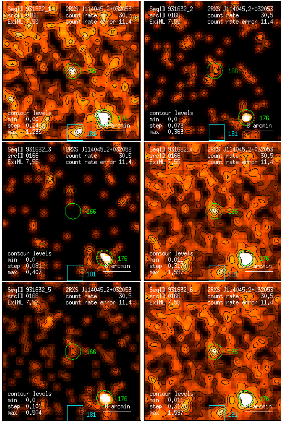
Figure 166: RASS 931632: detection 0166: band rate images, Gaussian filter: (1) PSPC channels 11 – 41, (2) 52 – 90, (3) 91 – 201, (4) 11 – 235, (5) 52 – 201, (6) 11 – 201. Broad band rates in counts/ks. Band rate contour levels in counts/ks/arcmin 2 .
