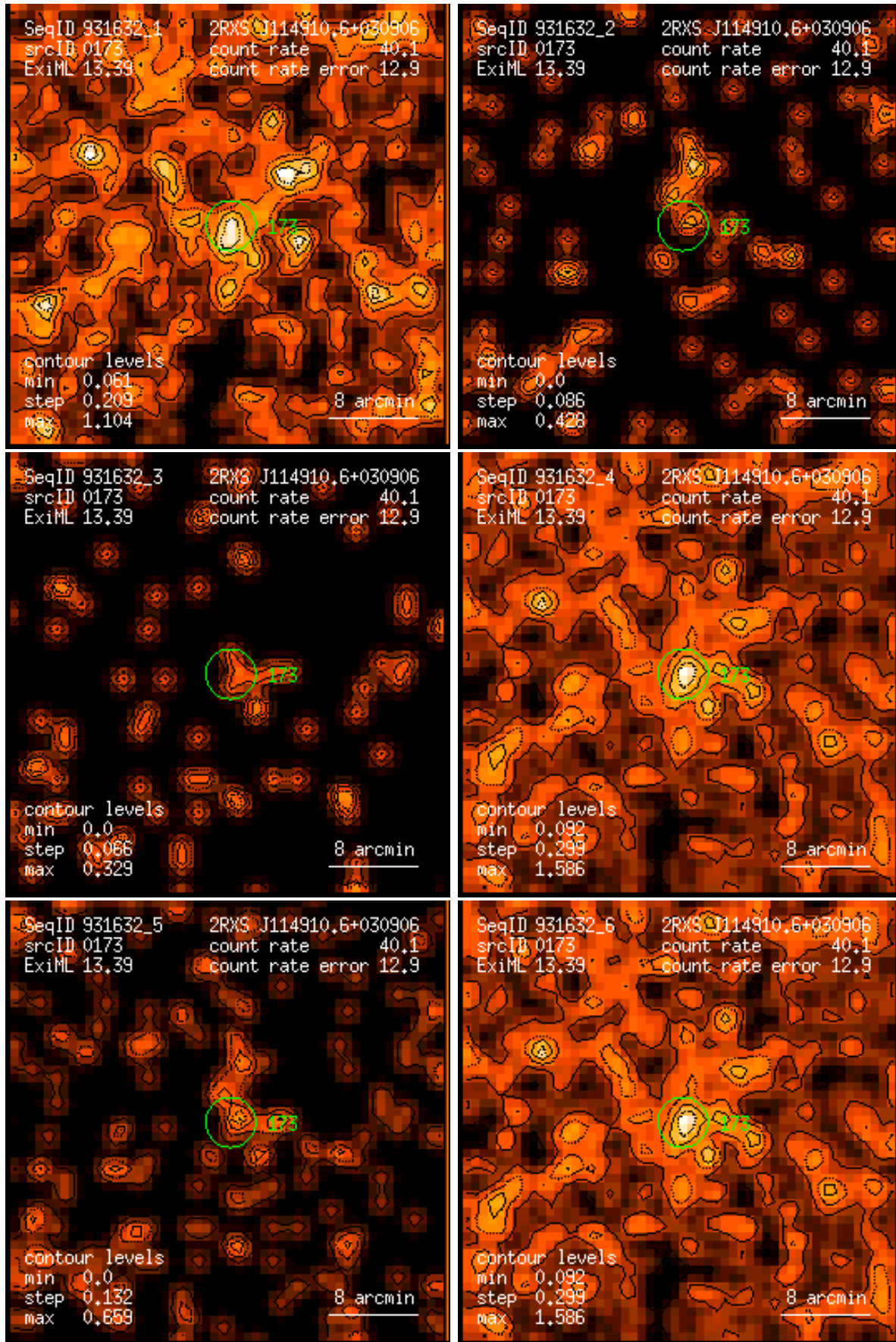
Figure 173: RASS 931632: detection 0173: band rate images, Gaussian filter: (1) PSPC channels 11 – 41, (2) 52 – 90, (3) 91 – 201, (4) 11 – 235, (5) 52 – 201, (6) 11 – 201. Broad band rates in counts/ks. Band rate contour levels in counts/ks/arcmin 2 .
