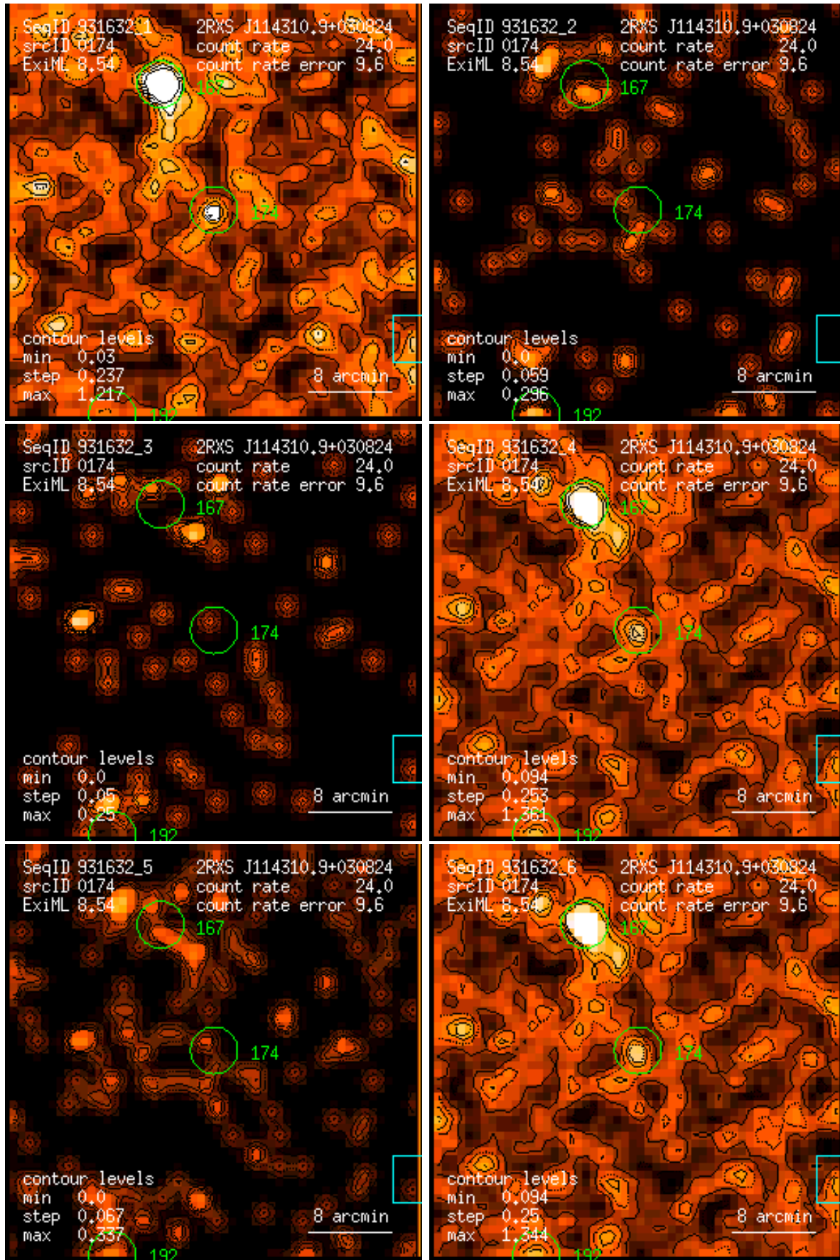
Figure 174: RASS 931632: detection 0174: band rate images, Gaussian filter: (1) PSPC channels 11 – 41, (2) 52 – 90, (3) 91 – 201, (4) 11 – 235, (5) 52 – 201, (6) 11 – 201. Broad band rates in counts/ks. Band rate contour levels in counts/ks/arcmin 2 .
