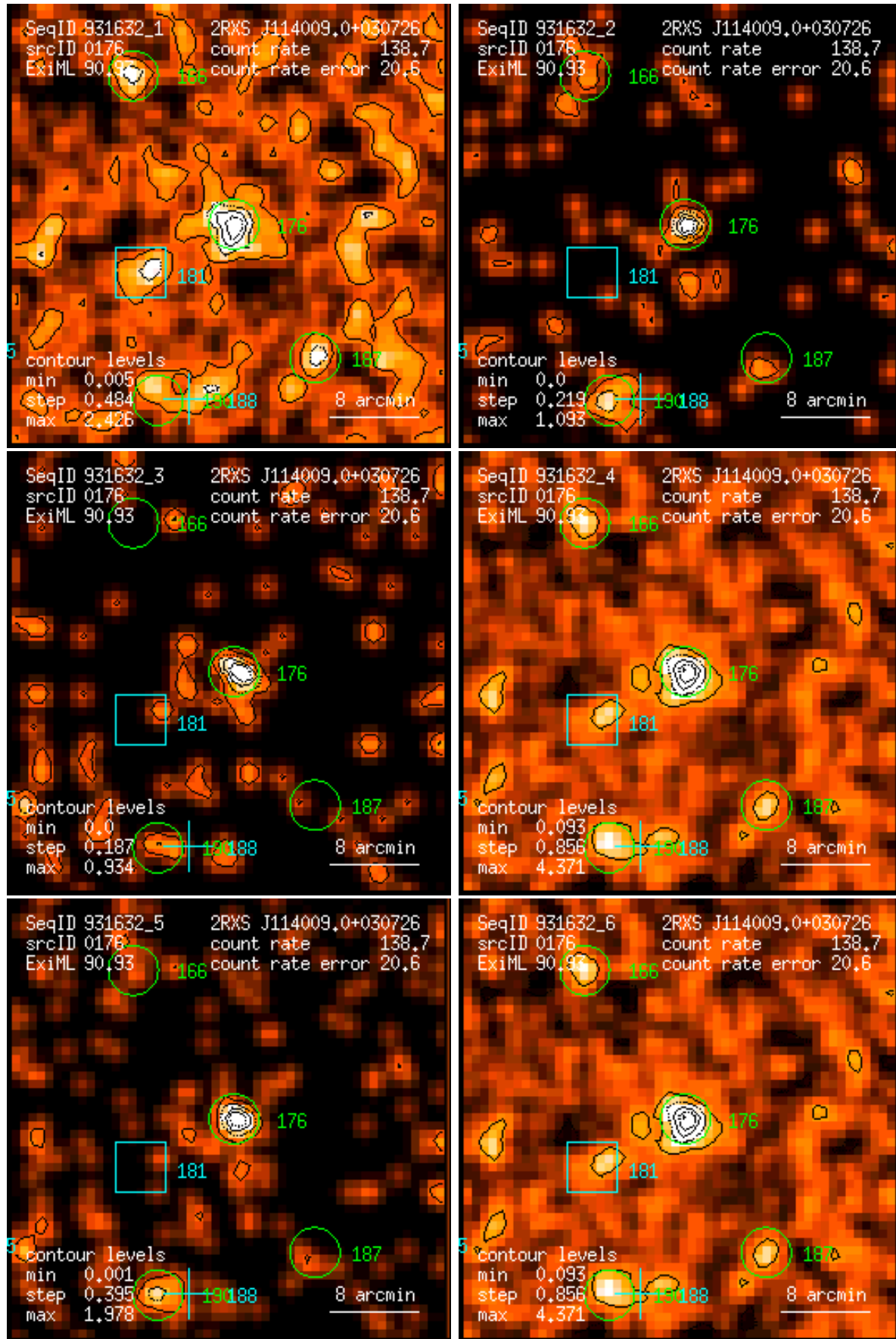
Figure 176: RASS 931632: detection 0176: band rate images, Gaussian filter: (1) PSPC channels 11 – 41, (2) 52 – 90, (3) 91 – 201, (4) 11 – 235, (5) 52 – 201, (6) 11 – 201. Broad band rates in counts/ks. Band rate contour levels in counts/ks/arcmin 2 .
