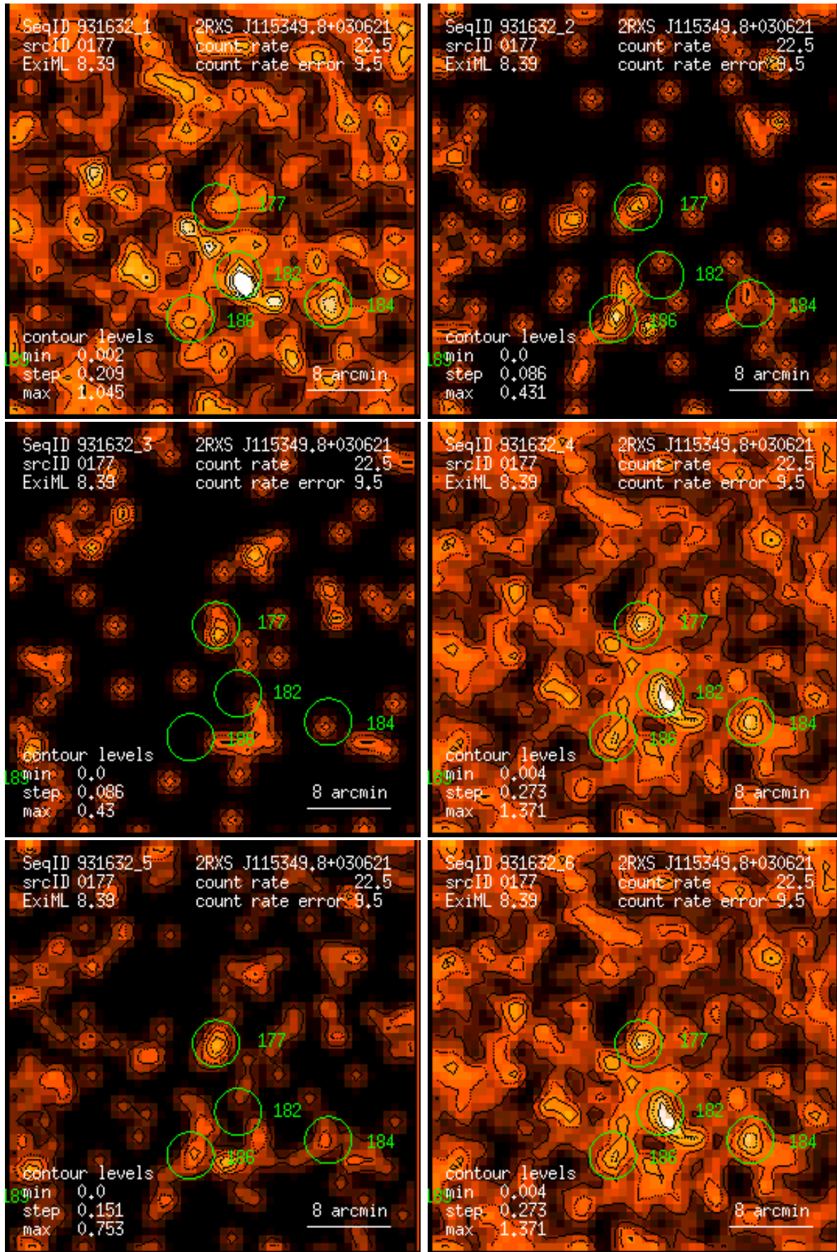
Figure 177: RASS 931632: detection 0177: band rate images, Gaussian filter: (1) PSPC channels 11 – 41, (2) 52 – 90, (3) 91 – 201, (4) 11 – 235, (5) 52 – 201, (6) 11 – 201. Broad band rates in counts/ks. Band rate contour levels in counts/ks/arcmin 2 .
