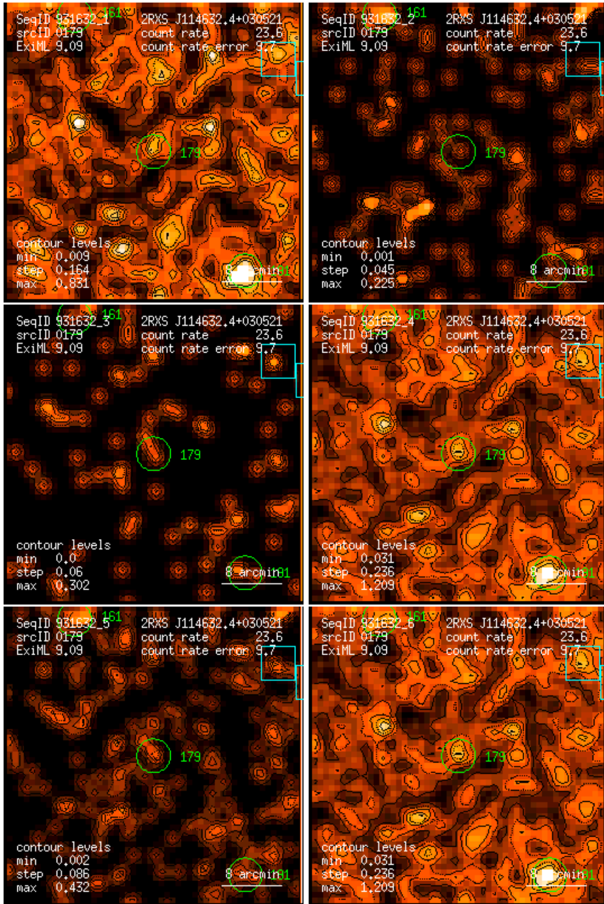
Figure 179: RASS 931632: detection 0179: band rate images, Gaussian filter: (1) PSPC channels 11 – 41, (2) 52 – 90, (3) 91 – 201, (4) 11 – 235, (5) 52 – 201, (6) 11 – 201. Broad band rates in counts/ks. Band rate contour levels in counts/ks/arcmin 2 .
