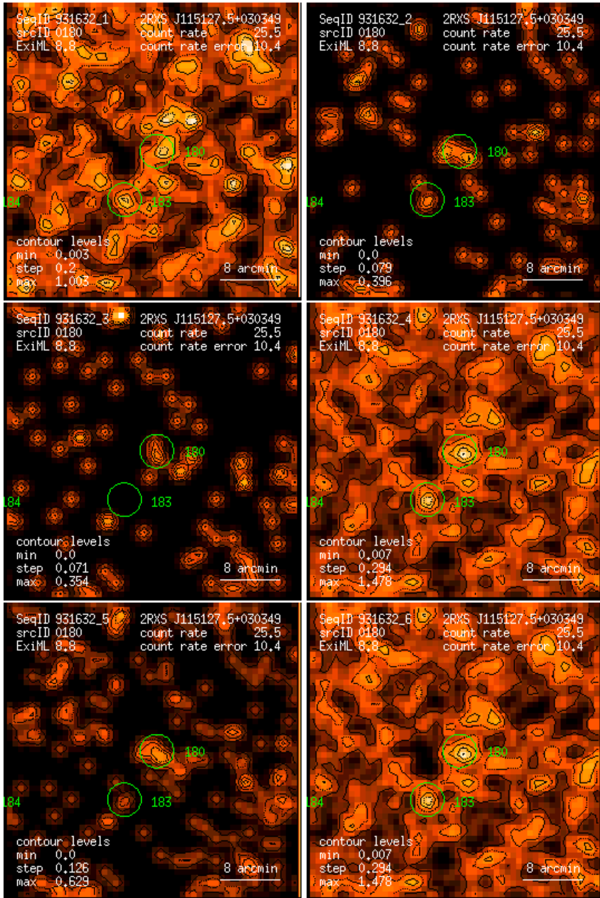
Figure 180: RASS 931632: detection 0180: band rate images, Gaussian filter: (1) PSPC channels 11 – 41, (2) 52 – 90, (3) 91 – 201, (4) 11 – 235, (5) 52 – 201, (6) 11 – 201. Broad band rates in counts/ks. Band rate contour levels in counts/ks/arcmin 2 .
