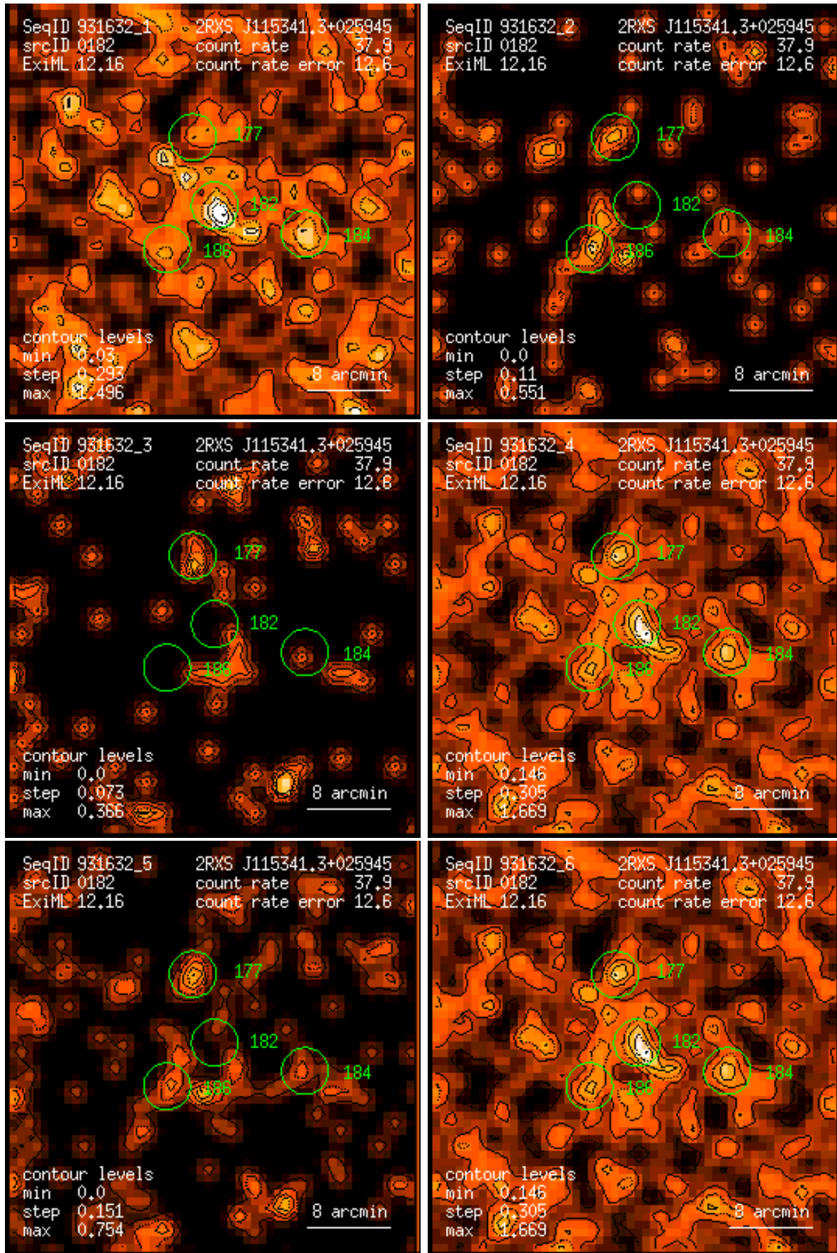
Figure 182: RASS 931632: detection 0182: band rate images, Gaussian filter: (1) PSPC channels 11 – 41, (2) 52 – 90, (3) 91 – 201, (4) 11 – 235, (5) 52 – 201, (6) 11 – 201. Broad band rates in counts/ks. Band rate contour levels in counts/ks/arcmin 2 .
