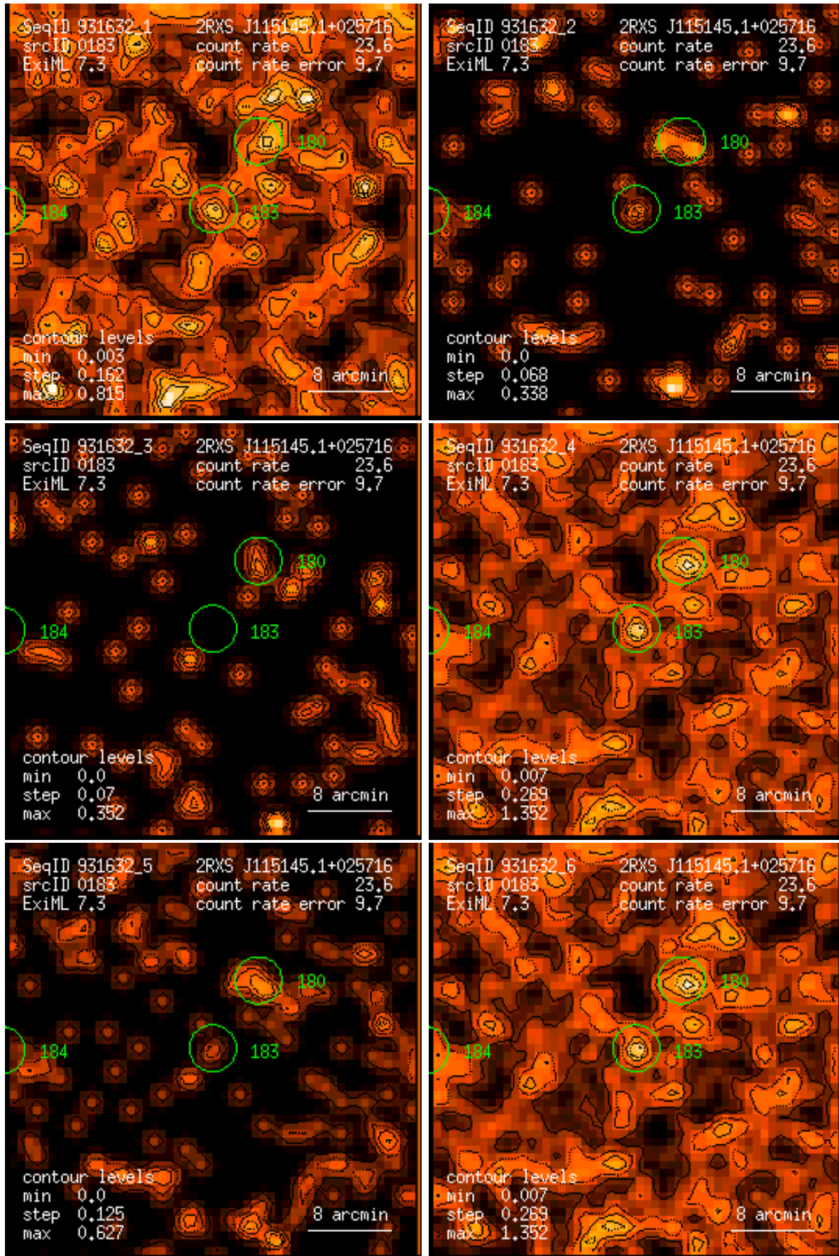
Figure 183: RASS 931632: detection 0183: band rate images, Gaussian filter: (1) PSPC channels 11 – 41, (2) 52 – 90, (3) 91 – 201, (4) 11 – 235, (5) 52 – 201, (6) 11 – 201. Broad band rates in counts/ks. Band rate contour levels in counts/ks/arcmin 2 .
