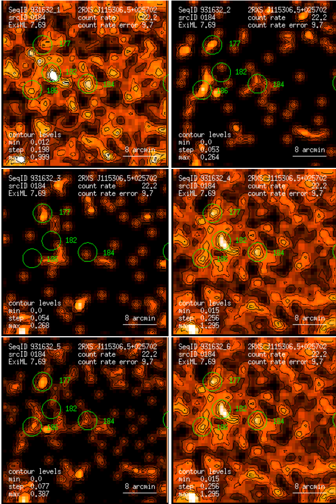
Figure 184: RASS 931632: detection 0184: band rate images, Gaussian filter: (1) PSPC channels 11 – 41, (2) 52 – 90, (3) 91 – 201, (4) 11 – 235, (5) 52 – 201, (6) 11 – 201. Broad band rates in counts/ks. Band rate contour levels in counts/ks/arcmin 2 .
