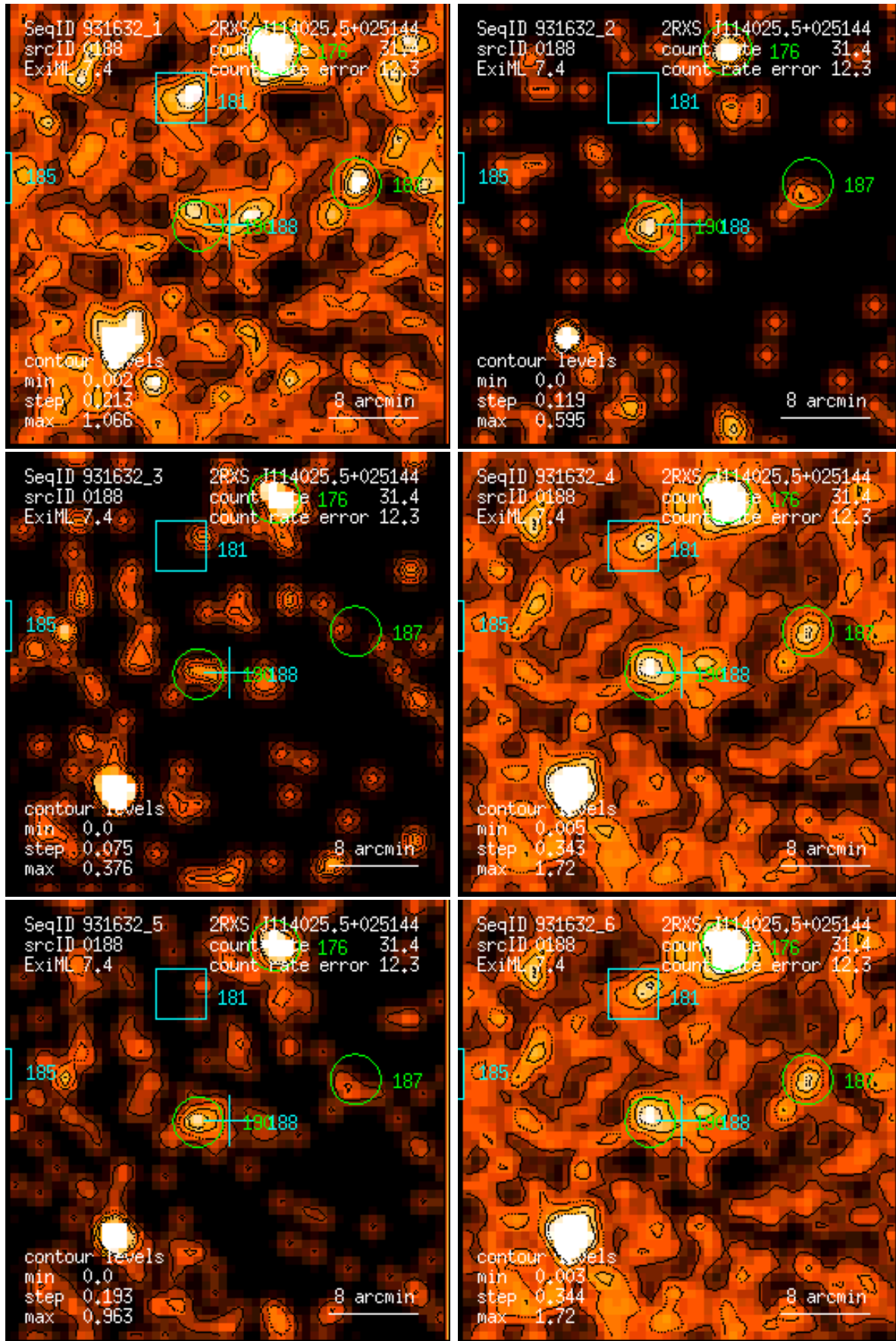
Figure 188: RASS 931632: detection 0188: band rate images, Gaussian filter: (1) PSPC channels 11 – 41, (2) 52 – 90, (3) 91 – 201, (4) 11 – 235, (5) 52 – 201, (6) 11 – 201. Broad band rates in counts/ks. Band rate contour levels in counts/ks/arcmin 2 .
