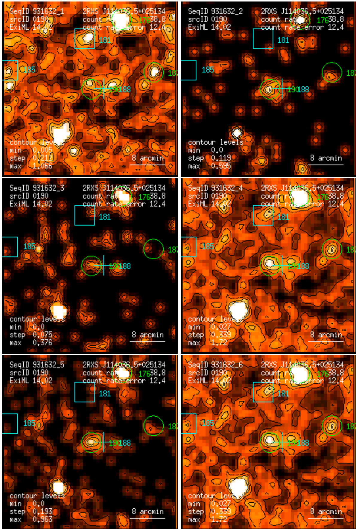
Figure 190: RASS 931632: detection 0190: band rate images, Gaussian filter: (1) PSPC channels 11 – 41, (2) 52 – 90, (3) 91 – 201, (4) 11 – 235, (5) 52 – 201, (6) 11 – 201. Broad band rates in counts/ks. Band rate contour levels in counts/ks/arcmin 2 .
