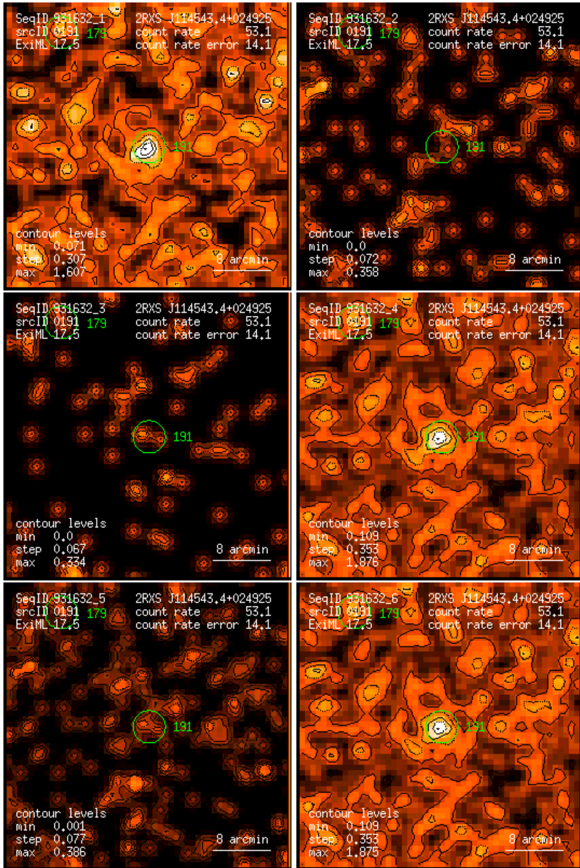
Figure 191: RASS 931632: detection 0191: band rate images, Gaussian filter: (1) PSPC channels 11 – 41, (2) 52 – 90, (3) 91 – 201, (4) 11 – 235, (5) 52 – 201, (6) 11 – 201. Broad band rates in counts/ks. Band rate contour levels in counts/ks/arcmin 2 .
