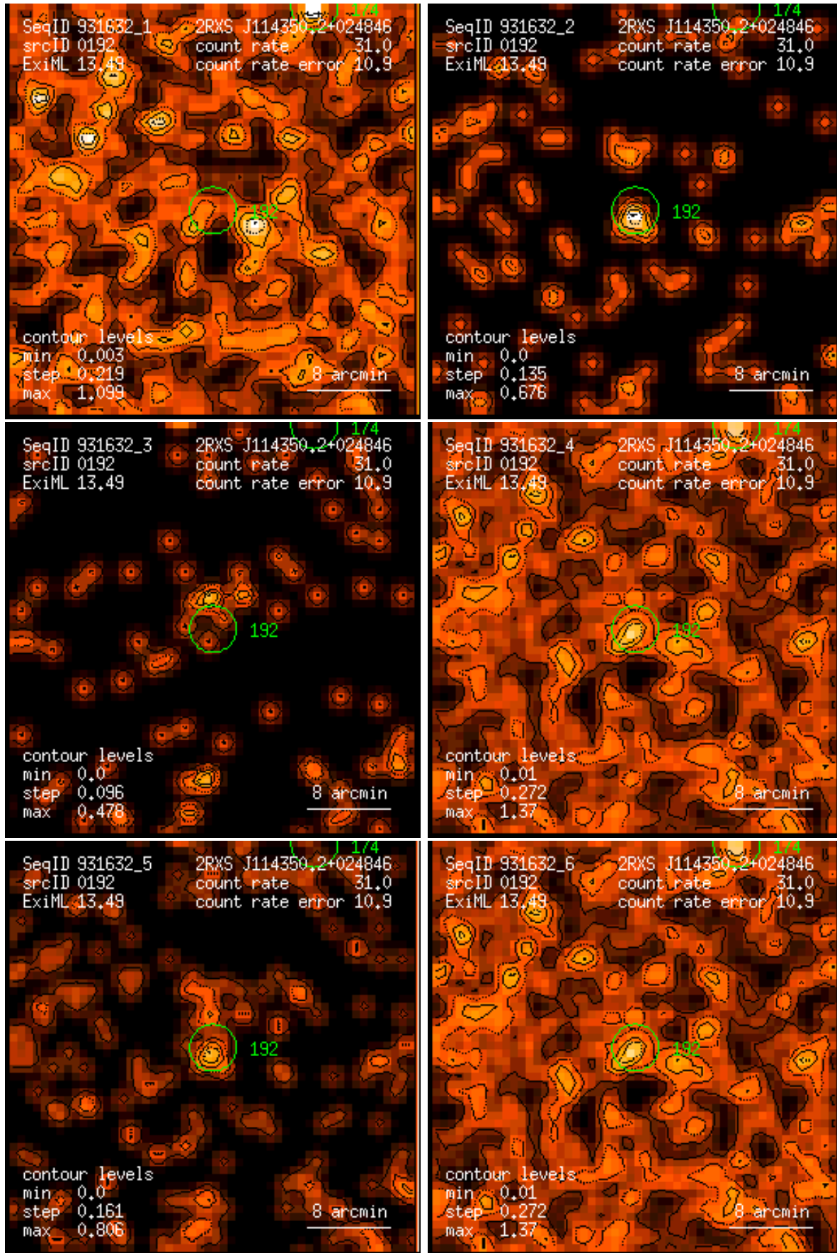
Figure 192: RASS 931632: detection 0192: band rate images, Gaussian filter: (1) PSPPC channels 11 – 41, (2) 52 – 90, (3) 91 – 201, (4) 11 – 235, (5) 52 – 201, (6) 11 – 201. Broad band rates in counts/ks. Band rate contour levels in counts/ks/arcmin 2 .
