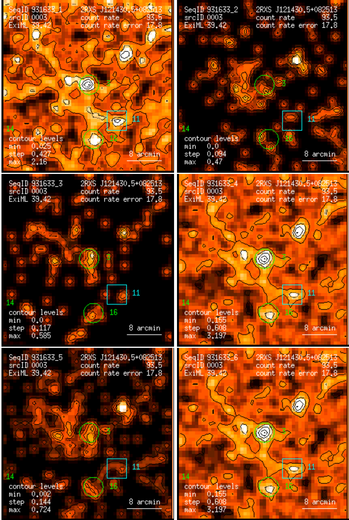
Figure 3: RASS 931633: detection 0003: band rate images, Gaussian filter: (1) PSPC channels 11 – 41, (2) 52 – 90, (3) 91 – 201, (4) 11 – 235, (5) 52 – 201, (6) 11 – 201. Broad band rates in counts/ks. Band rate contour levels in counts/ks/arcmin 2 .
