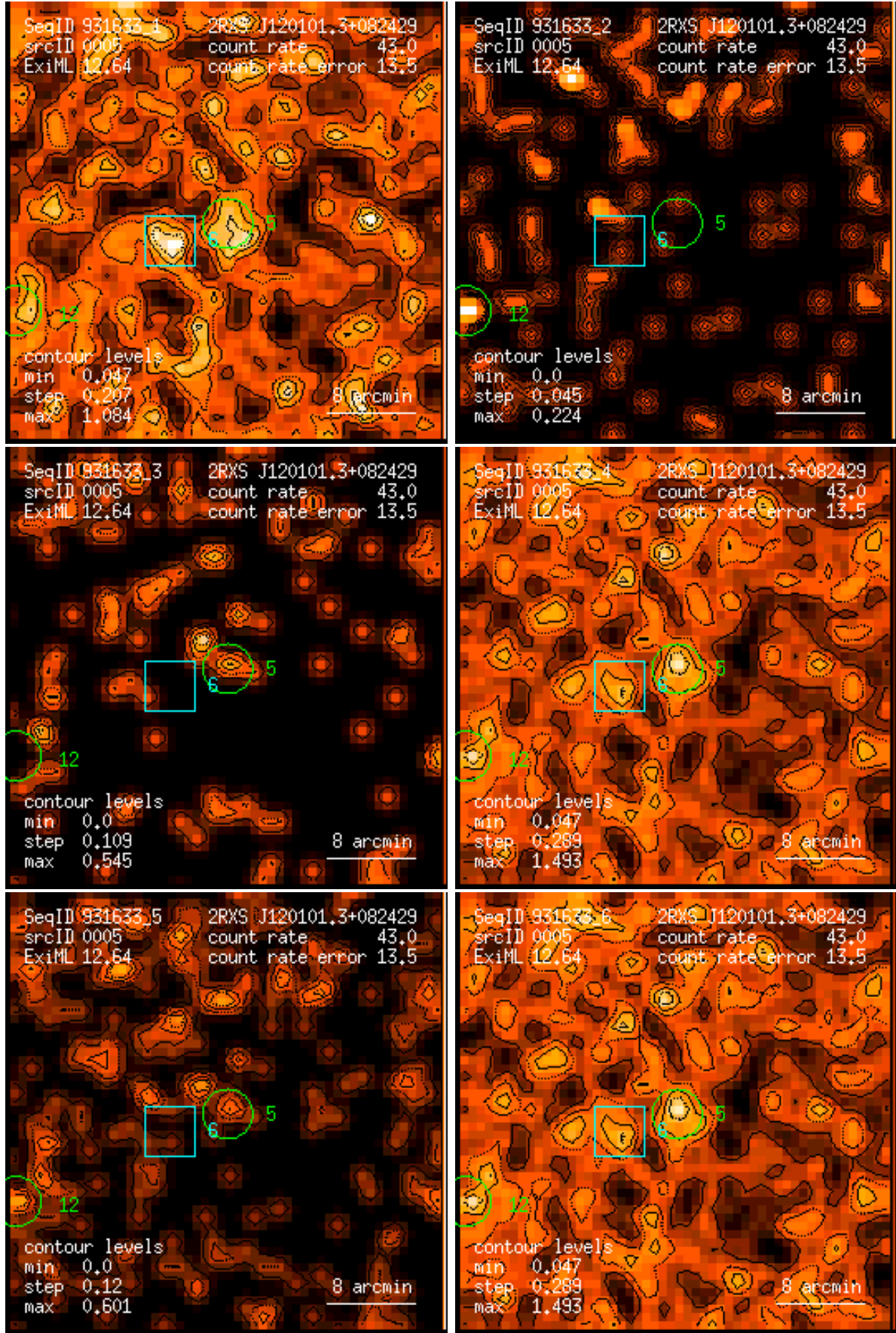
Figure 5: RASS 931633: detection 0005: band rate images, Gaussian filter: (1) PSPC channels 11 – 41, (2) 52 – 90, (3) 91 – 201, (4) 11 – 235, (5) 52 – 201, (6) 11 – 201. Broad band rates in counts/ks. Band rate contour levels in counts/ks/arcmin 2 .
