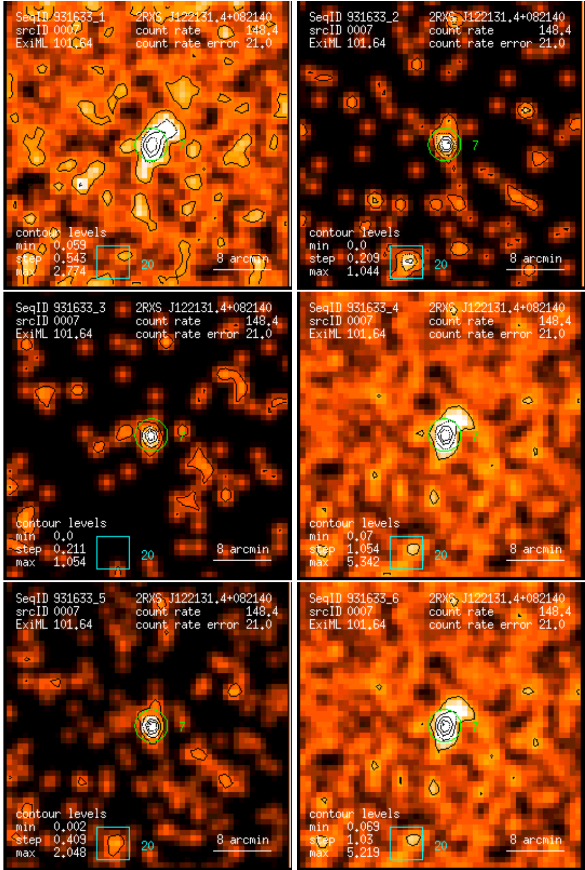
Figure 7: RASS 931633: detection 0007: band rate images, Gaussian filter: (1) PSPC channels 11 – 41, (2) 52 – 90, (3) 91 – 201, (4) 11 – 235, (5) 52 – 201, (6) 11 – 201. Broad band rates in counts/ks. Band rate contour levels in counts/ks/arcmin 2 .
