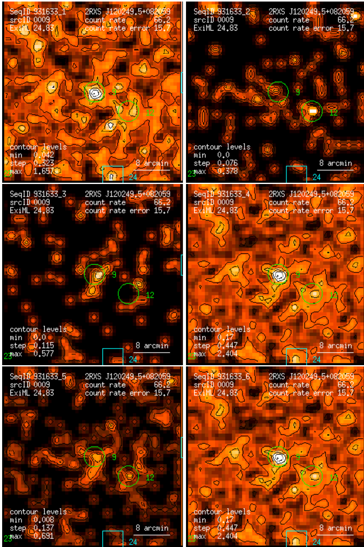
Figure 9: RASS 931633: detection 0009: band rate images, Gaussian filter: (1) PSPC channels 11 – 41, (2) 52 – 90, (3) 91 – 201, (4) 11 – 235, (5) 52 – 201, (6) 11 – 201. Broad band rates in counts/ks. Band rate contour levels in counts/ks/arcmin 2 .
