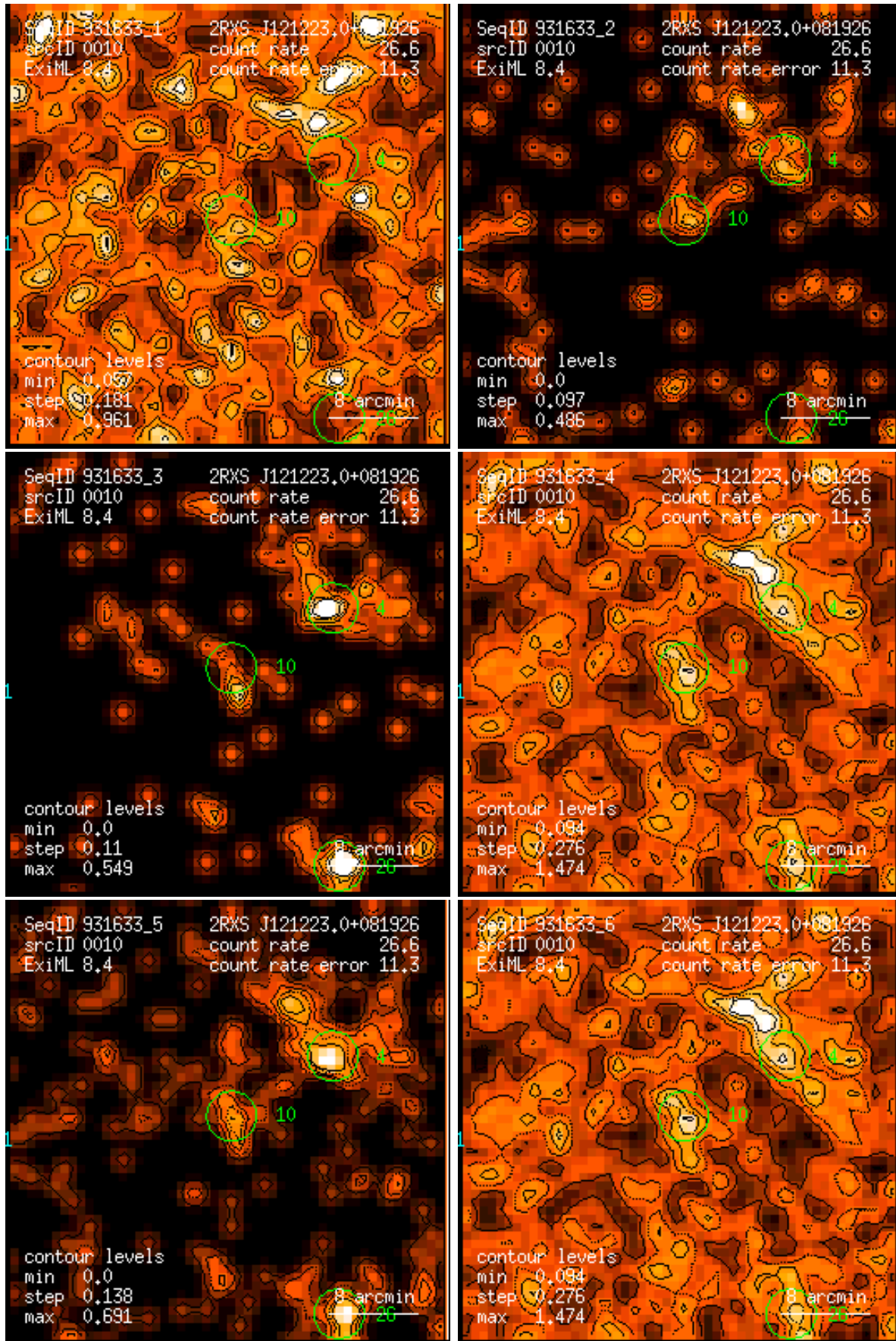
Figure 10: RASS 931633: detection 0010: band rate images, Gaussian filter: (1) PSPC channels 11 – 41, (2) 52 – 90, (3) 91 – 201, (4) 11 – 235, (5) 52 – 201, (6) 11 – 201. Broad band rates in counts/ks. Band rate contour levels in counts/ks/arcmin 2 .
