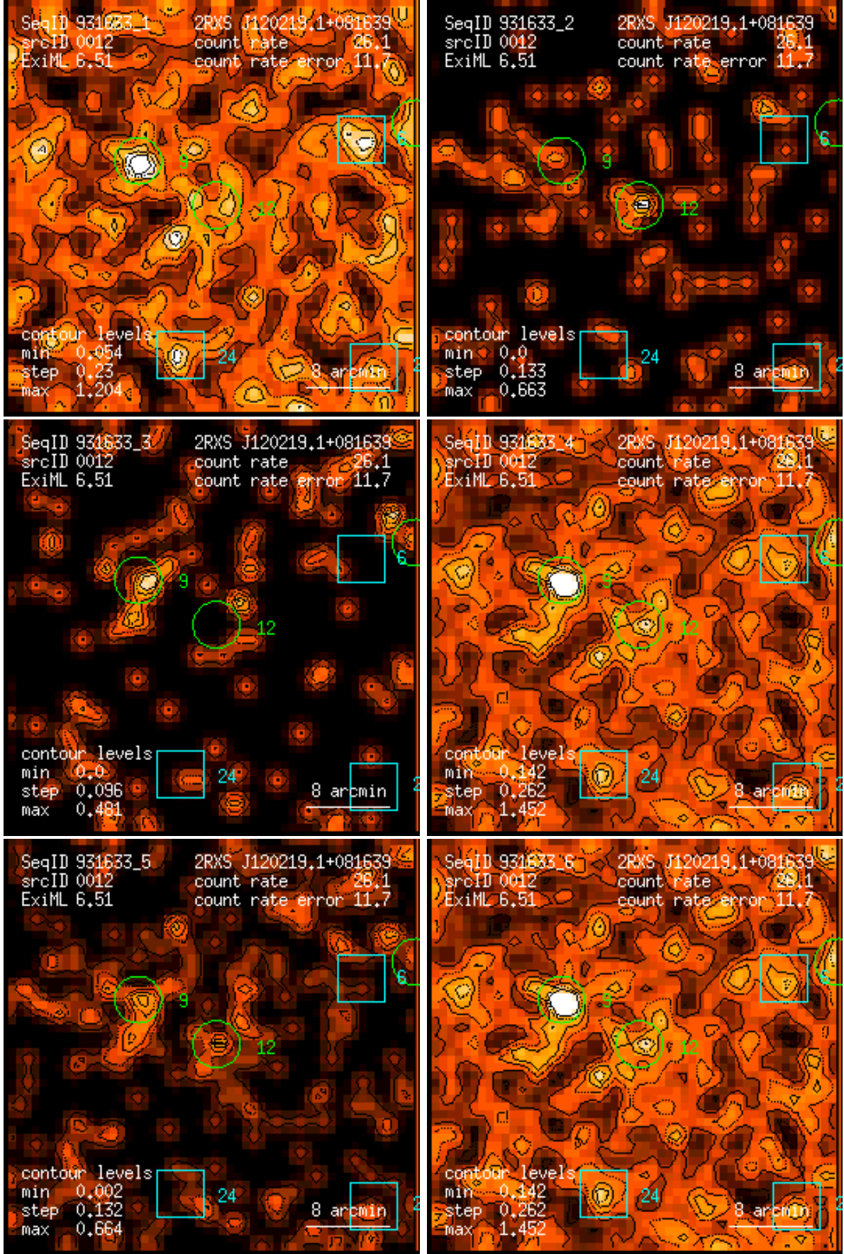
Figure 12: RASS 931633: detection 0012: band rate images, Gaussian filter: (1) PSPC channels 11 – 41, (2) 52 – 90, (3) 91 – 201, (4) 11 – 235, (5) 52 – 201, (6) 11 – 201. Broad band rates in counts/ks. Band rate contour levels in counts/ks/arcmin 2 .
