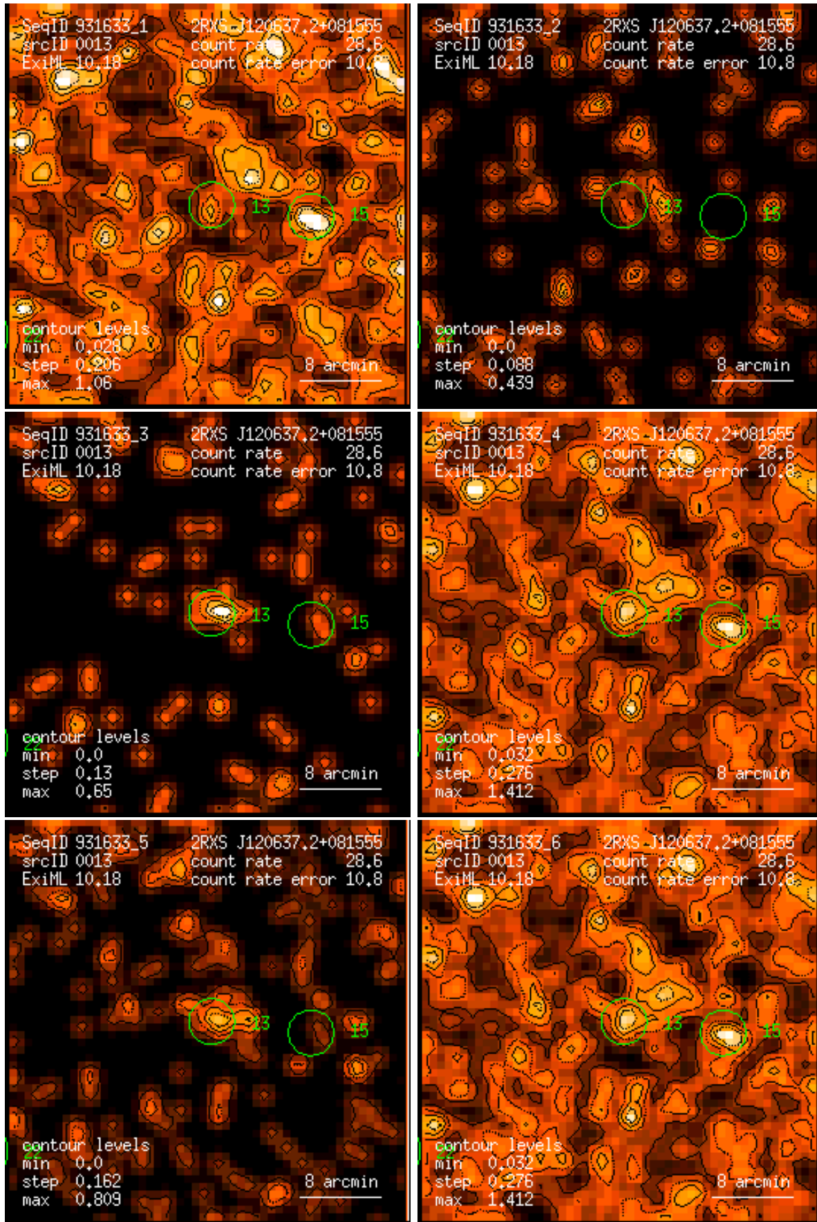
Figure 13: RASS 931633: detection 0013: band rate images, Gaussian filter: (1) PSPC channels 11 – 41, (2) 52 – 90, (3) 91 – 201, (4) 11 – 235, (5) 52 – 201, (6) 11 – 201. Broad band rates in counts/ks. Band rate contour levels in counts/ks/arcmin 2 .
