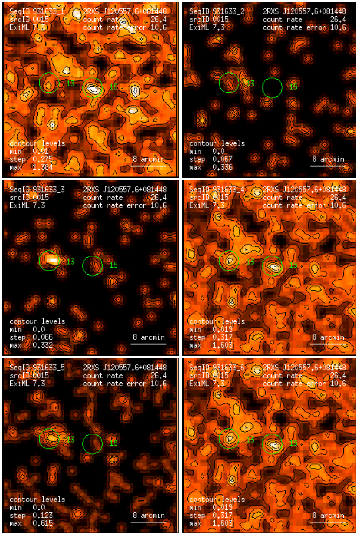
Figure 15: RASS 931633: detection 0015: band rate images, Gaussian filter: (1) PSPC channels 11 – 41, (2) 52 – 90, (3) 91 – 201, (4) 11 – 235, (5) 52 – 201, (6) 11 – 201. Broad band rates in counts/ks. Band rate contour levels in counts/ks/arcmin 2 .
