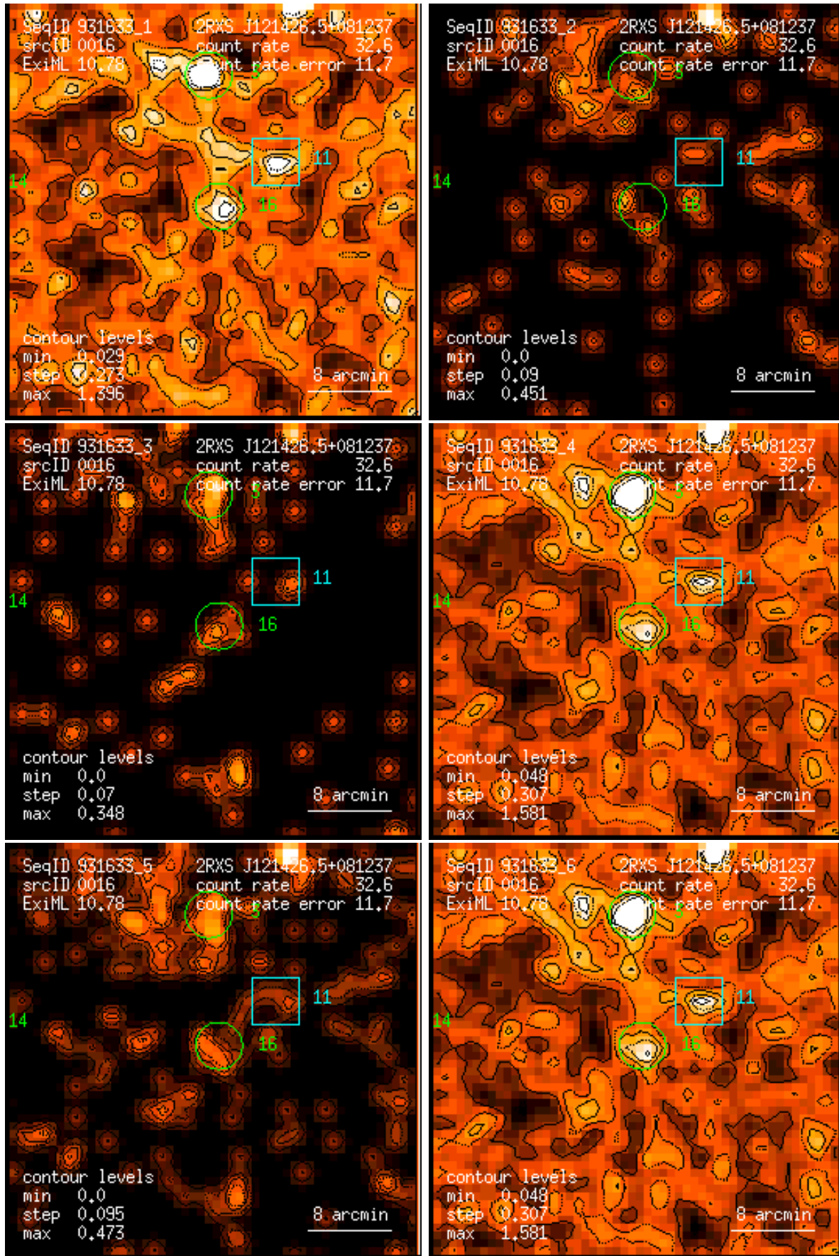
Figure 16: RASS 931633: detection 0016: band rate images, Gaussian filter: (1) PSPC channels 11 – 41, (2) 52 – 90, (3) 91 – 201, (4) 11 – 235, (5) 52 – 201, (6) 11 – 201. Broad band rates in counts/ks. Band rate contour levels in counts/ks/arcmin 2 .
