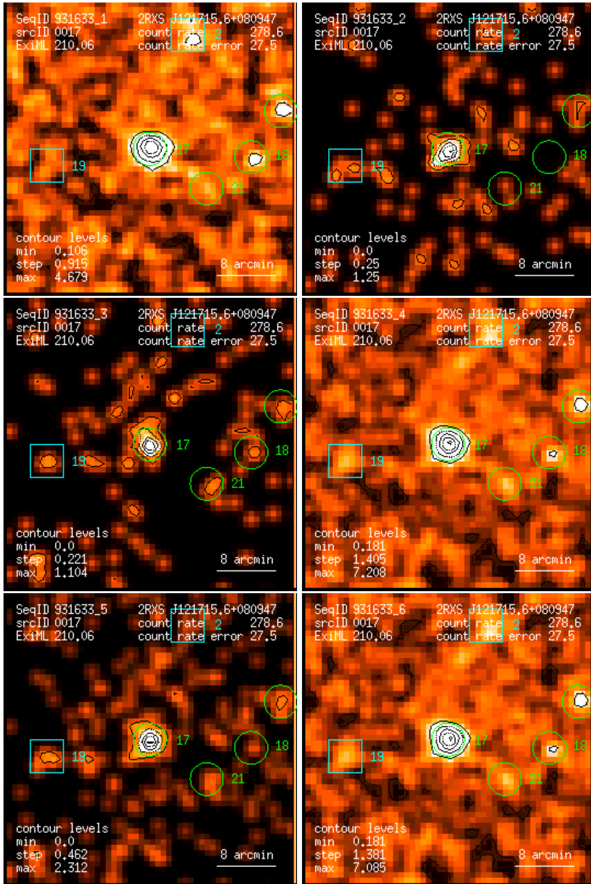
Figure 17: RASS 931633: detection 0017: band rate images, Gaussian filter: (1) PSPC channels 11 – 41, (2) 52 – 90, (3) 91 – 201, (4) 11 – 235, (5) 52 – 201, (6) 11 – 201. Broad band rates in counts/ks. Band rate contour levels in counts/ks/arcmin 2 .
