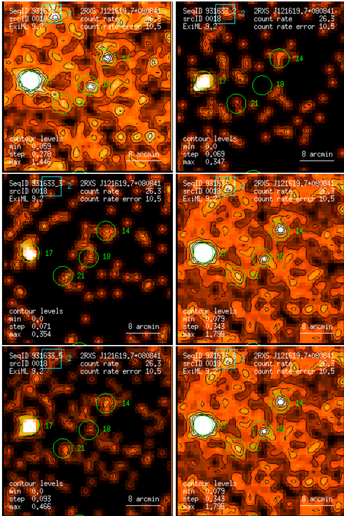
Figure 18: RASS 931633: detection 0018: band rate images, Gaussian filter: (1) PSPC channels 11 – 41, (2) 52 – 90, (3) 91 – 201, (4) 11 – 235, (5) 52 – 201, (6) 11 – 201. Broad band rates in counts/ks. Band rate contour levels in counts/ks/arcmin 2 .
