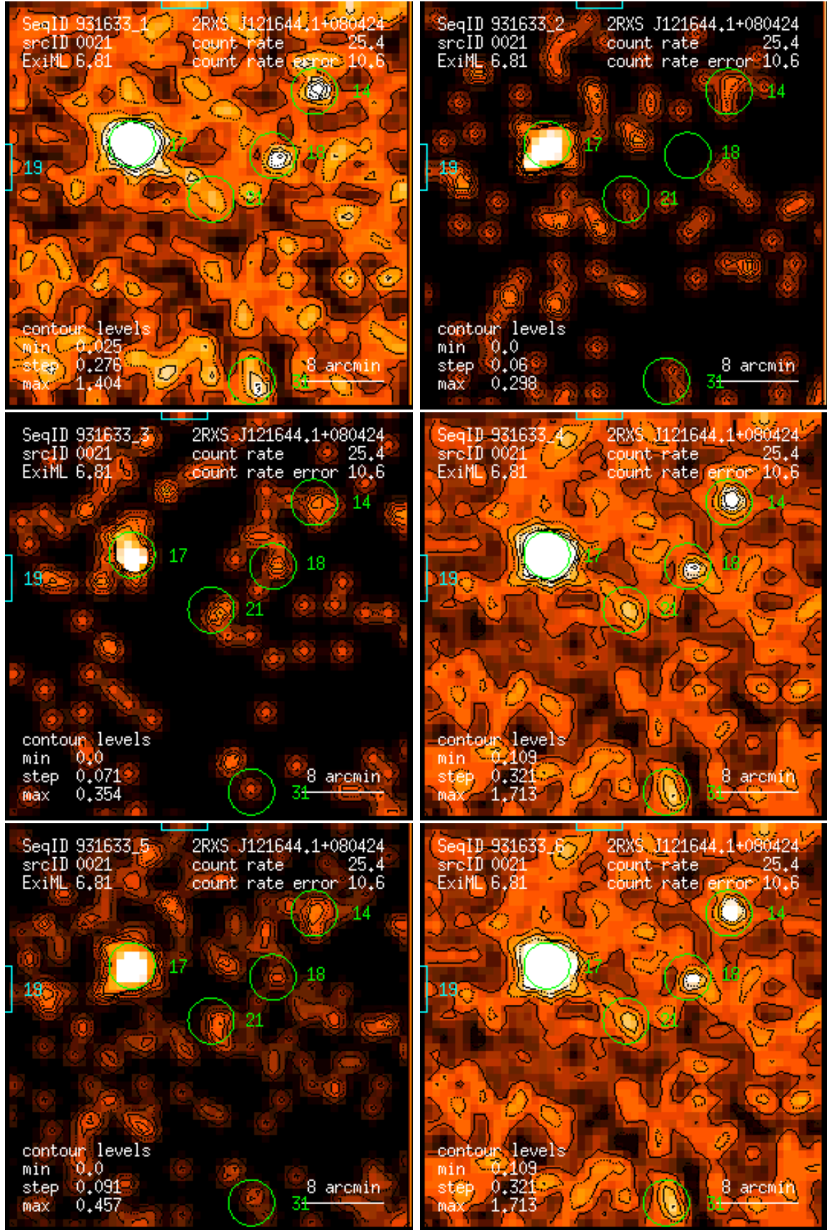
Figure 21: RASS 931633: detection 0021: band rate images, Gaussian filter: (1) PSPC channels 11 – 41, (2) 52 – 90, (3) 91 – 201, (4) 11 – 235, (5) 52 – 201, (6) 11 – 201. Broad band rates in counts/ks. Band rate contour levels in counts/ks/arcmin 2 .
