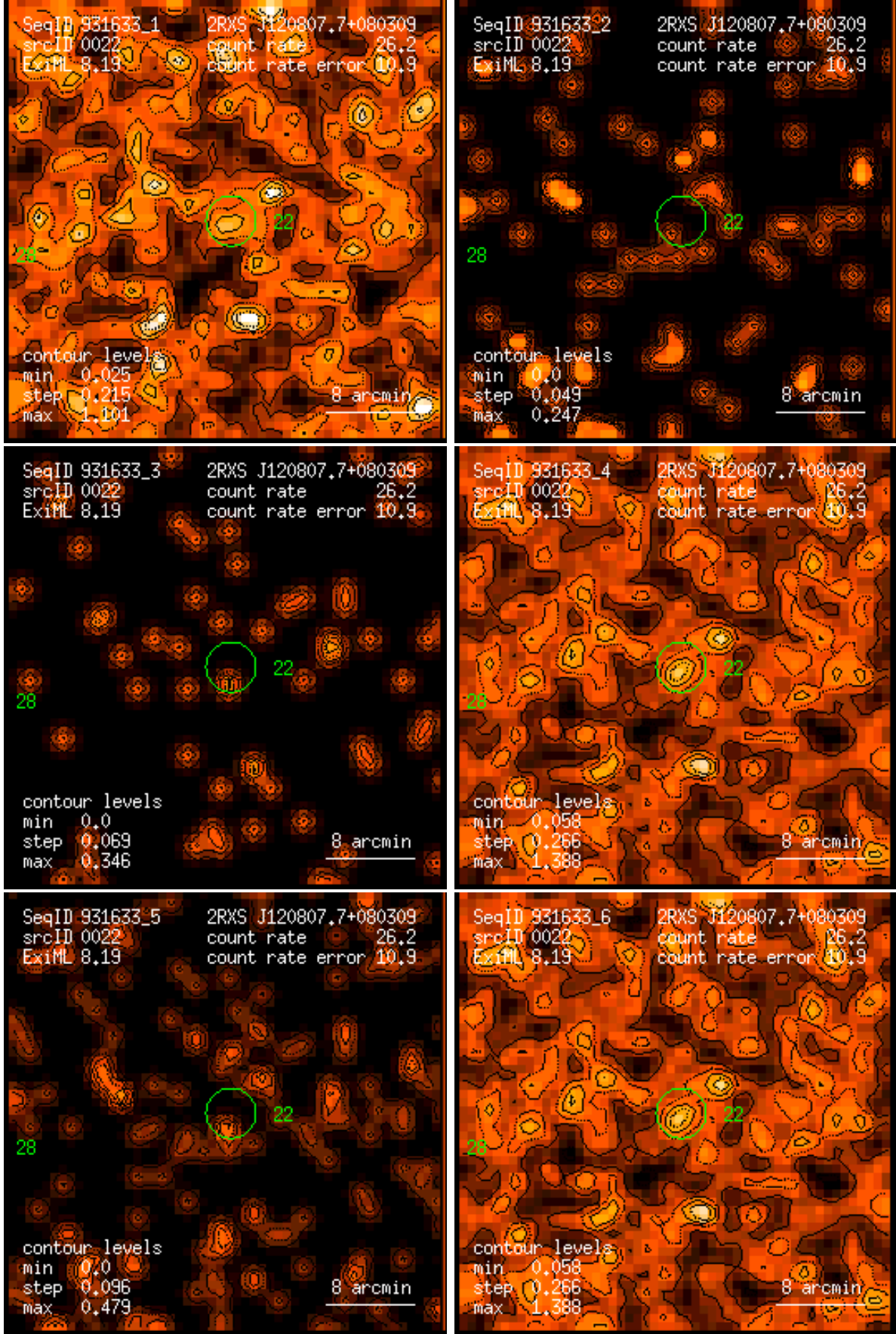
Figure 22: RASS 931633: detection 0022: band rate images, Gaussian filter: (1) PSPC channels 11 – 41, (2) 52 – 90, (3) 91 – 201, (4) 11 – 235, (5) 52 – 201, (6) 11 – 201. Broad band rates in counts/ks. Band rate contour levels in counts/ks/arcmin 2 .
