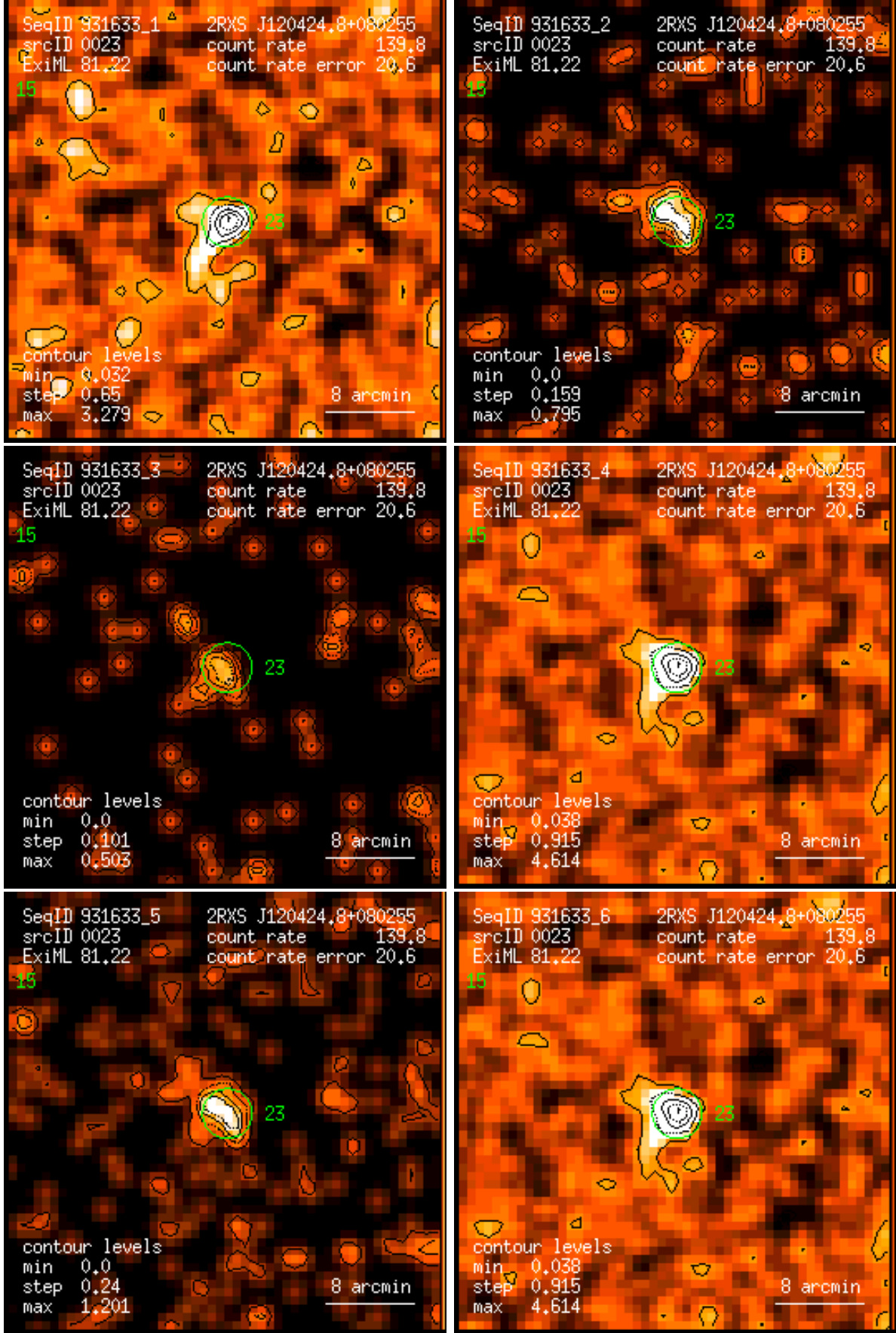
Figure 23: RASS 931633: detection 0023: band rate images, Gaussian filter: (1) PSPC channels 11 – 41, (2) 52 – 90, (3) 91 – 201, (4) 11 – 235, (5) 52 – 201, (6) 11 – 201. Broad band rates in counts/ks. Band rate contour levels in counts/ks/arcmin 2 .
