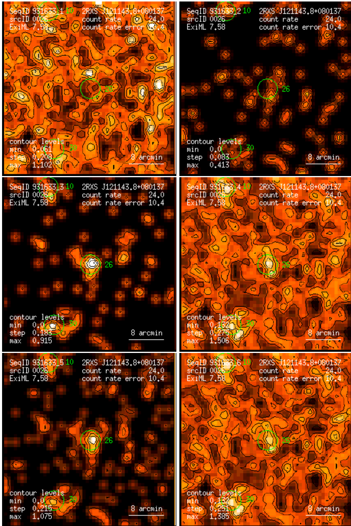
Figure 26: RASS 931633: detection 0026: band rate images, Gaussian filter: (1) PSPC channels 11 – 41, (2) 52 – 90, (3) 91 – 201, (4) 11 – 235, (5) 52 – 201, (6) 11 – 201. Broad band rates in counts/ks. Band rate contour levels in counts/ks/arcmin 2 .
