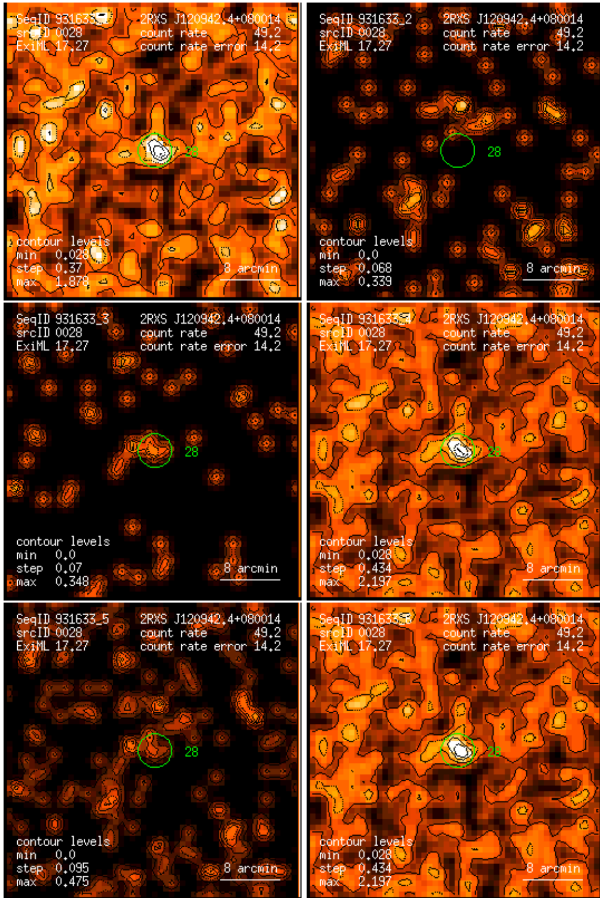
Figure 28: RASS 931633: detection 0028: band rate images, Gaussian filter: (1) PSPC channels 11 – 41, (2) 52 – 90, (3) 91 – 201, (4) 11 – 235, (5) 52 – 201, (6) 11 – 201. Broad band rates in counts/ks. Band rate contour levels in counts/ks/arcmin 2 .
