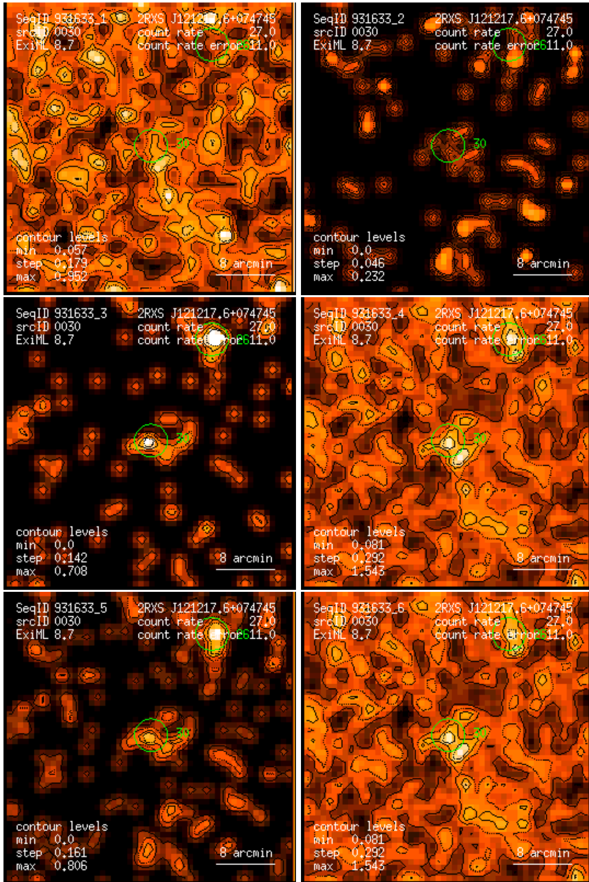
Figure 30: RASS 931633: detection 0030: band rate images, Gaussian filter: (1) PSPC channels 11 – 41, (2) 52 – 90, (3) 91 – 201, (4) 11 – 235, (5) 52 – 201, (6) 11 – 201. Broad band rates in counts/ks. Band rate contour levels in counts/ks/arcmin 2 .
