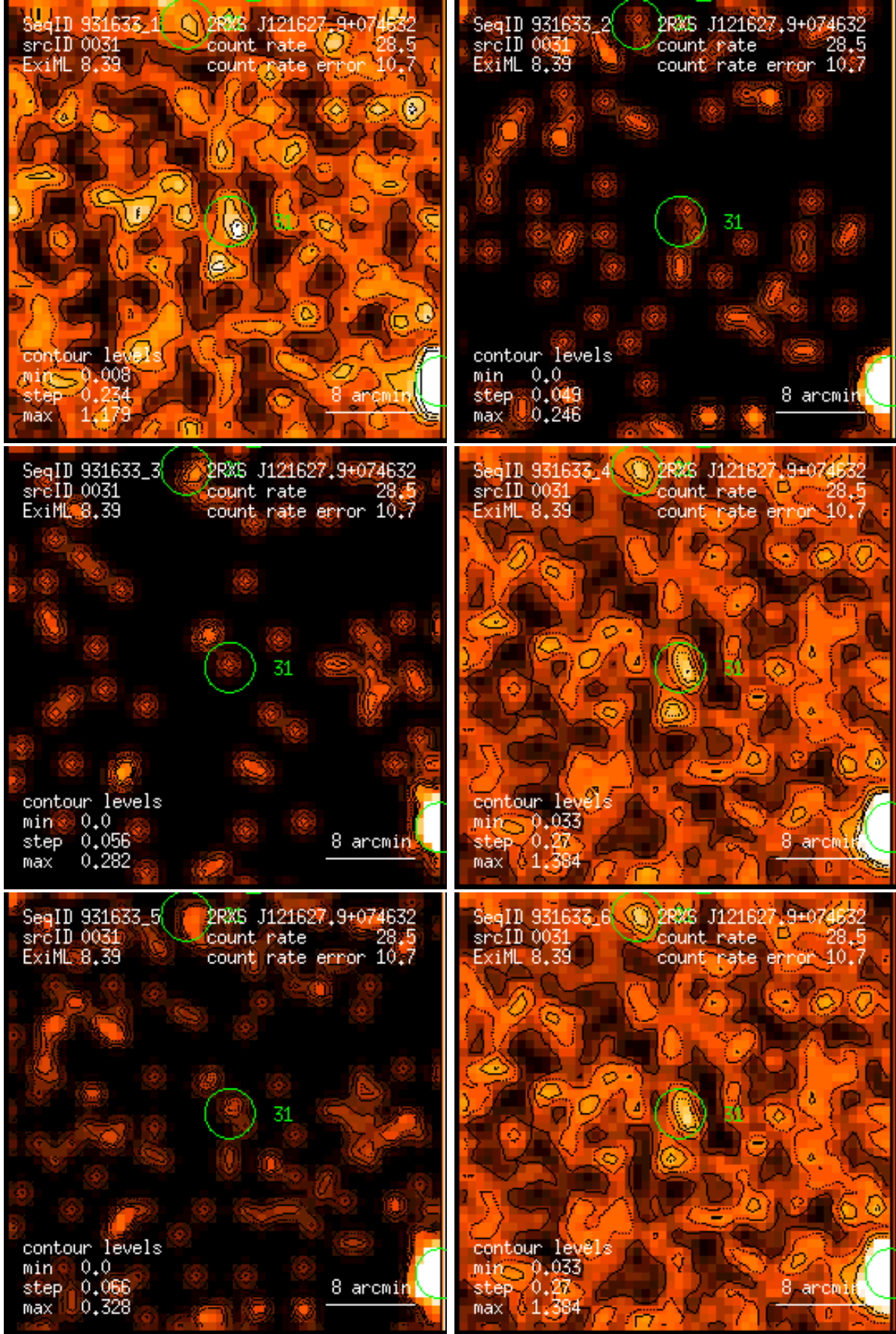
Figure 31: RASS 931633: detection 0031: band rate images, Gaussian filter: (1) PSPC channels 11 – 41, (2) 52 – 90, (3) 91 – 201, (4) 11 – 235, (5) 52 – 201, (6) 11 – 201. Broad band rates in counts/ks. Band rate contour levels in counts/ks/arcmin 2 .
